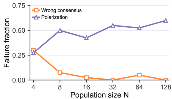
b) Failure decomposition by N
