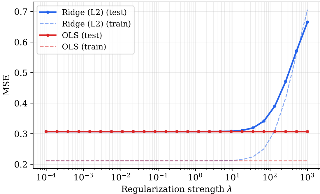
Synthetic — Train / Test MSE vs \lambda
