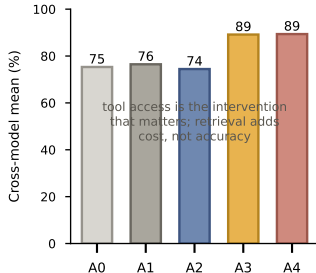
Corrected rerun, all four models
