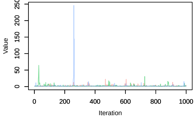
Trace – alpha_angles[3]
