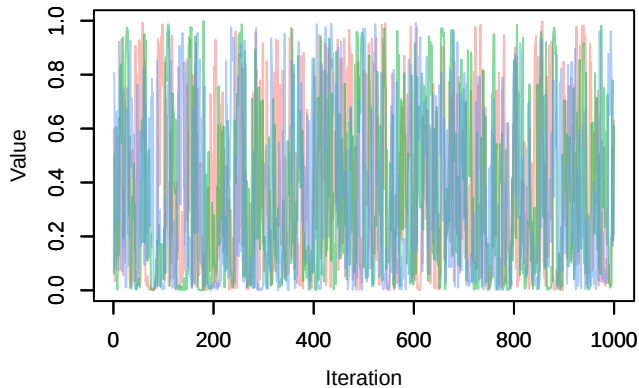
Trace – weights[1]
