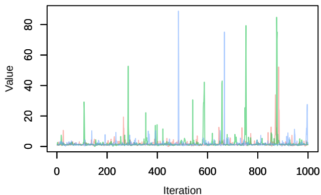
Trace – beta_angles[2]
