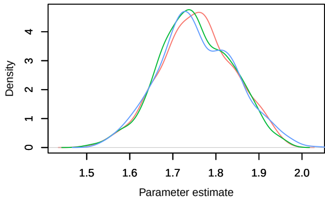
Density – dep
