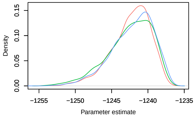
Density – alpha
