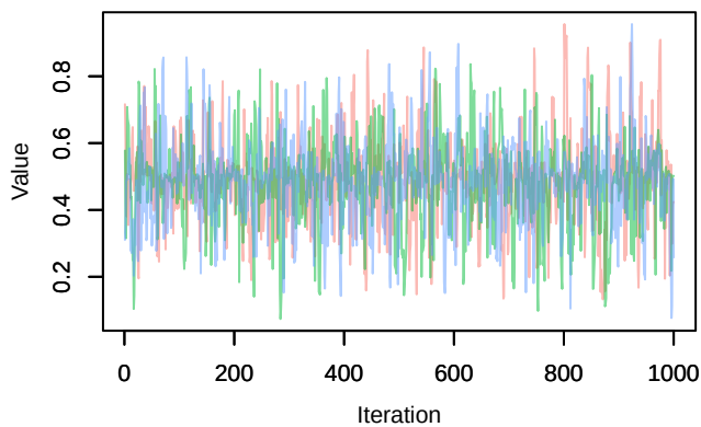
Trace – mu[3]
