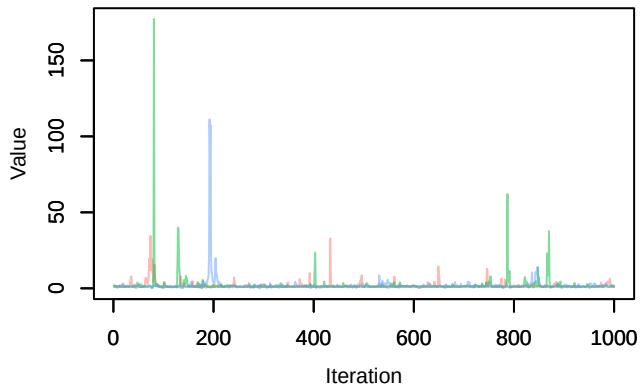
Trace – alpha_angles[2]
