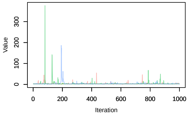
Trace – tau[2]
