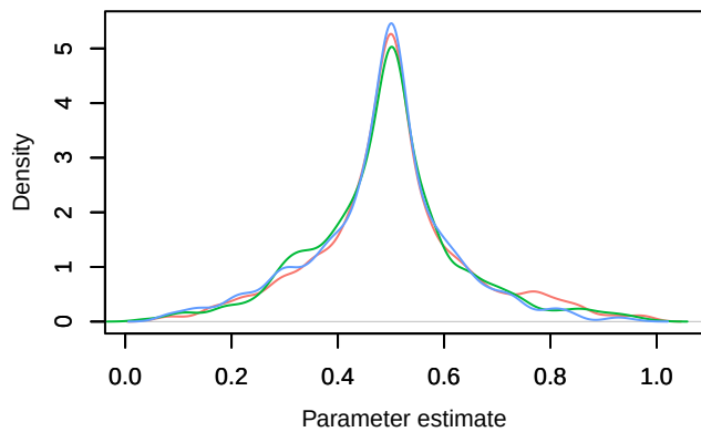
Density – mu[3]
