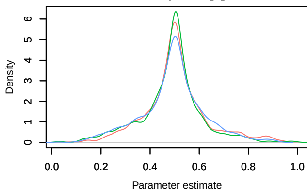
Density – mu[2]
