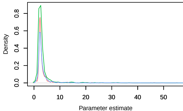
Density – tau[2]
