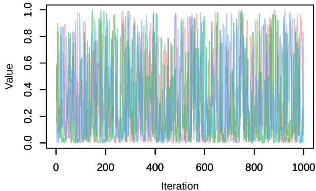
Trace – weights[3]
