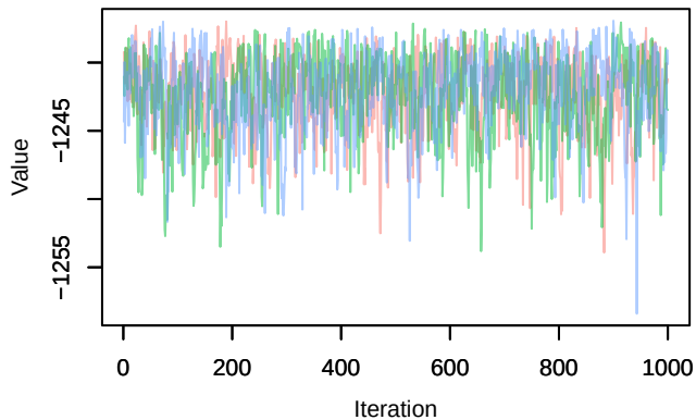
Trace – alpha
