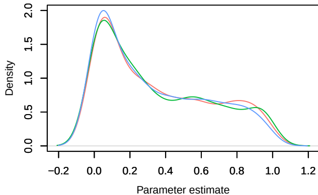
Density – weights[1]
