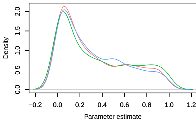
Density – weights[2]
