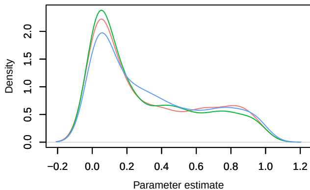
Density – weights[3]
