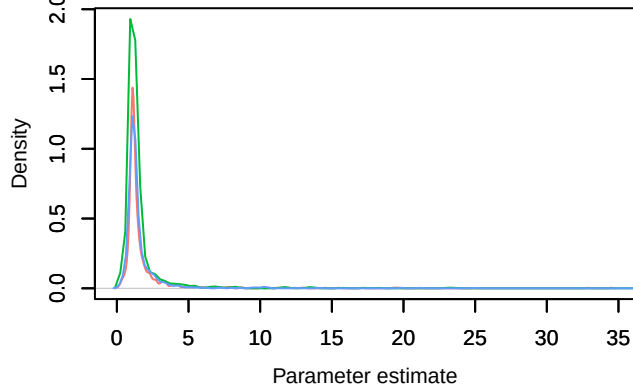
Density – alpha_angles[2]
