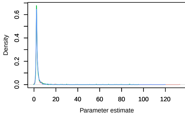
Density – tau[3]
