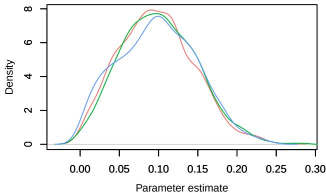
Density – dep
