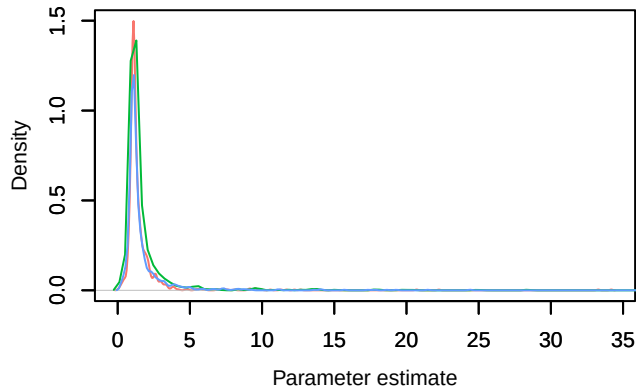
Density – beta_angles[2]
