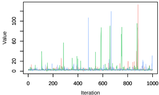
Trace – tau[3]
