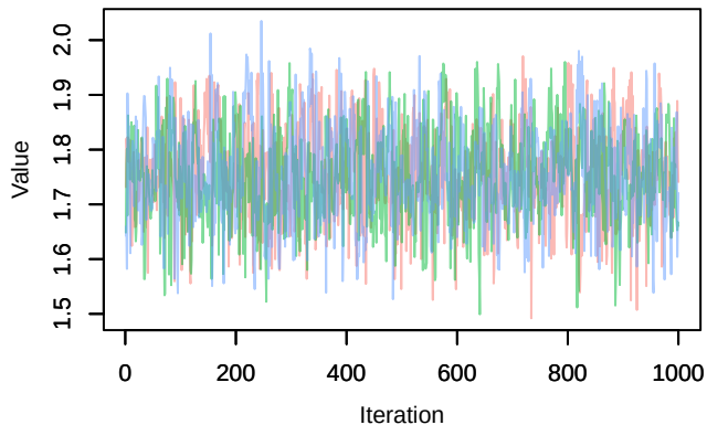
Trace – dep
