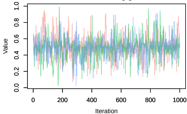
Trace – mu[2]
