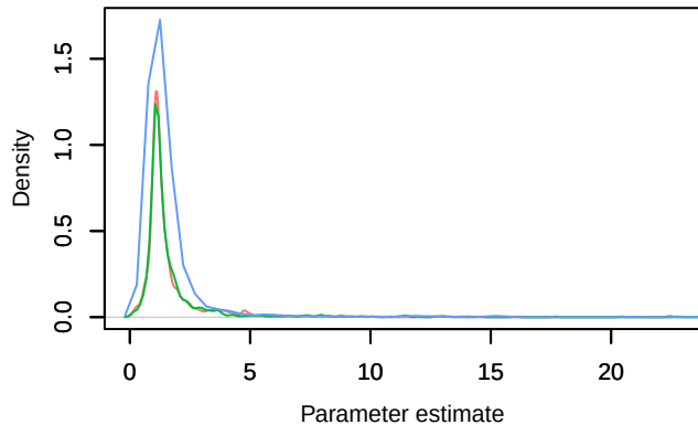
Density – alpha_angles[3]
