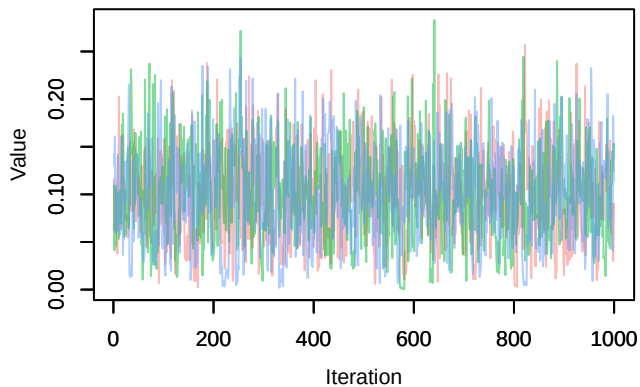
Trace – dep
