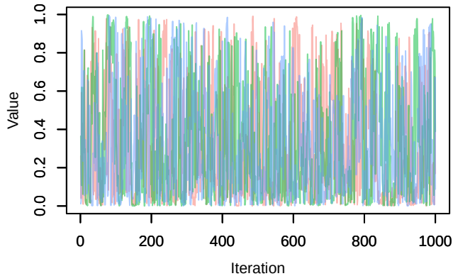
Trace – weights[2]
