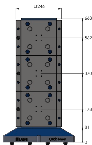
Tower 70650, height 668 mm, max. 3 pallets on each face.
