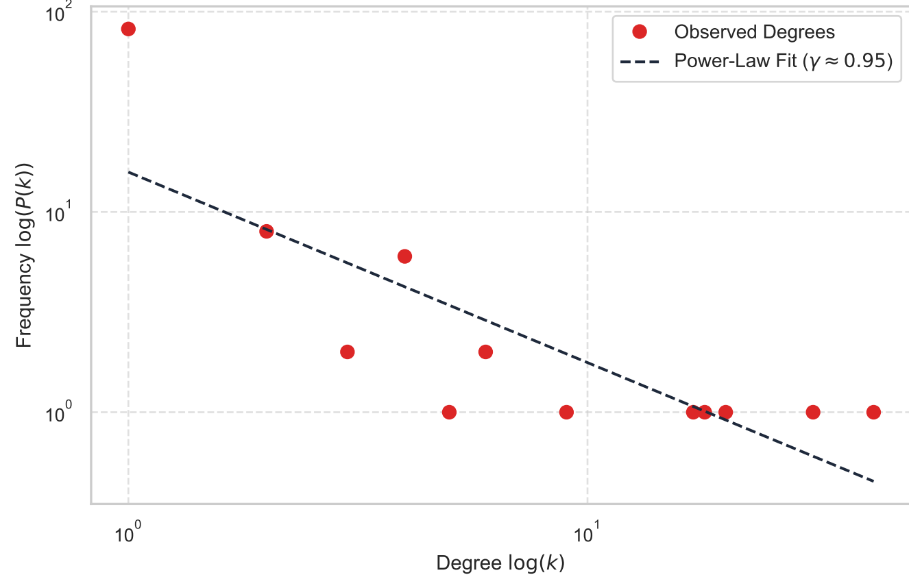
Log-Log Degree Distribution (Exploratory Power-Law Fit)
