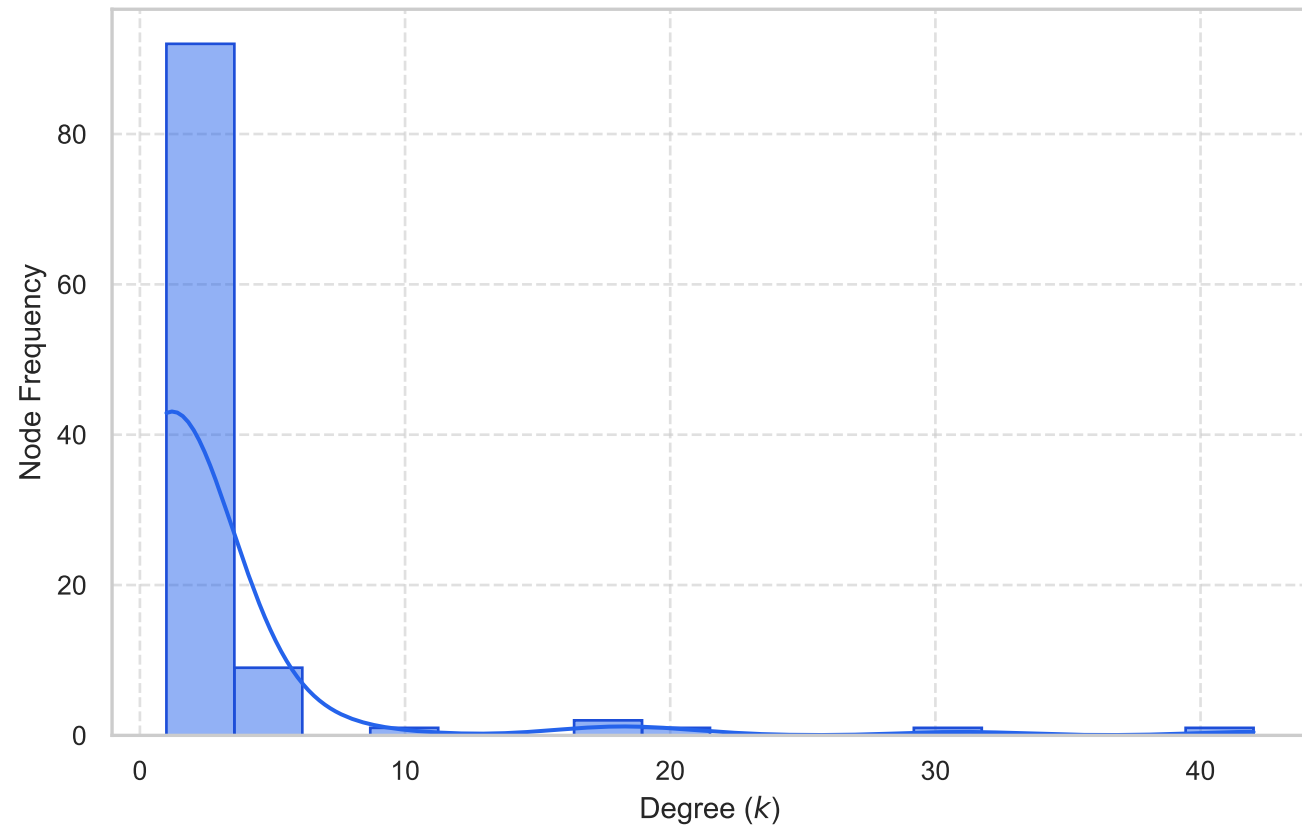
Node Degree Frequency Distribution
