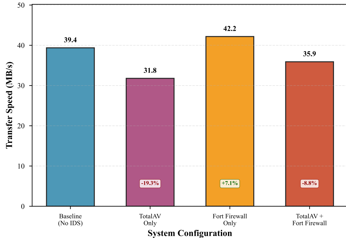
Criterion E: SMB Local Network Transfer
