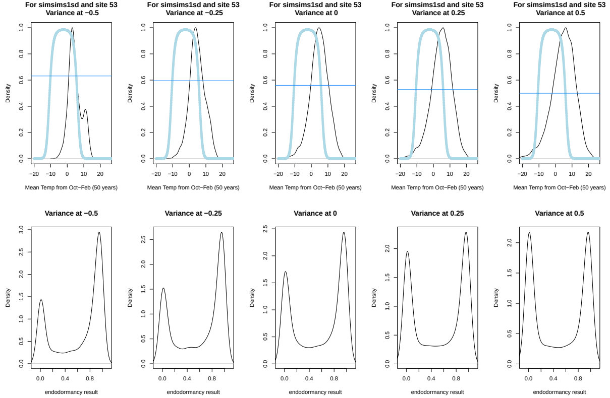
Figure 19: Top: Pinus endodormancy curves (same curve, always in light blue) across mean temperatures with changing variance at 53°N latitude. Darker blue horizontal line shows estimated endodormancy. Because of which side the endodormancy curve is on relative to temperature, increasing variance leads to more days falling outside the curve and leading to (bottom) 0 accumulated endodormancy, instead of 1.
