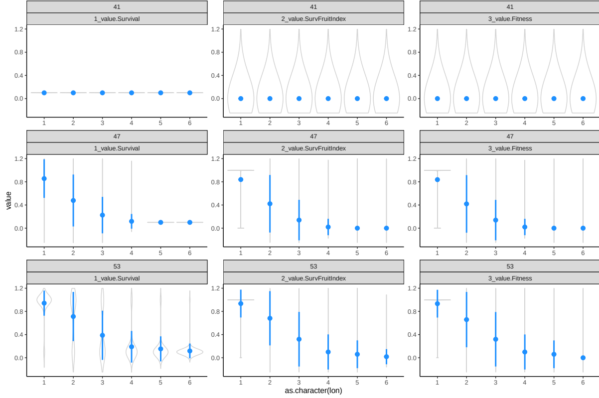
Figure 5: Pinus across 0 (1) to +5 (6) mean warming showing three latitudes. There is no survival at low latitudes, while at higher latitudes (see Fig. ??) warming leads to lower fitness due to low carbon survival (not enough chilling, so late dormancy break).
