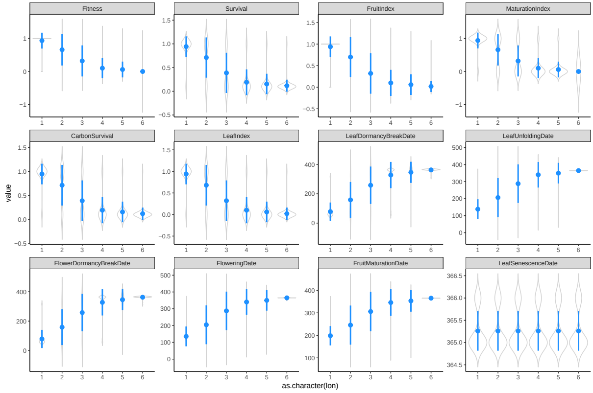
Figure 7: Pinus across 0 (1) to +5 (6) mean warming across fitness components at 53°N latitude. See notes in caption of Fig. ??.
