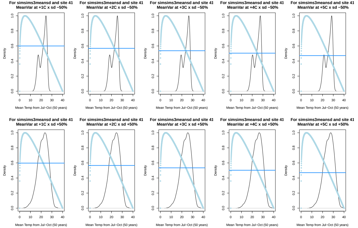
Figure 21: Top: Fagus fruit maturation curves (same curve, always in light blue, black is the daily temperatures) across changing mean temperatures with changing variance at 53°N latitude. Darker blue horizontal line shows estimated endodormancy. You can see declines in estimated endodormancy with increasing mean and variance, which explains stalling (or getting later) FruitMat with increasing mean and variance (see also issue 13). This is one of two curves in this process, but the only one likely to do anything interesting (as the other is sigmoid).
