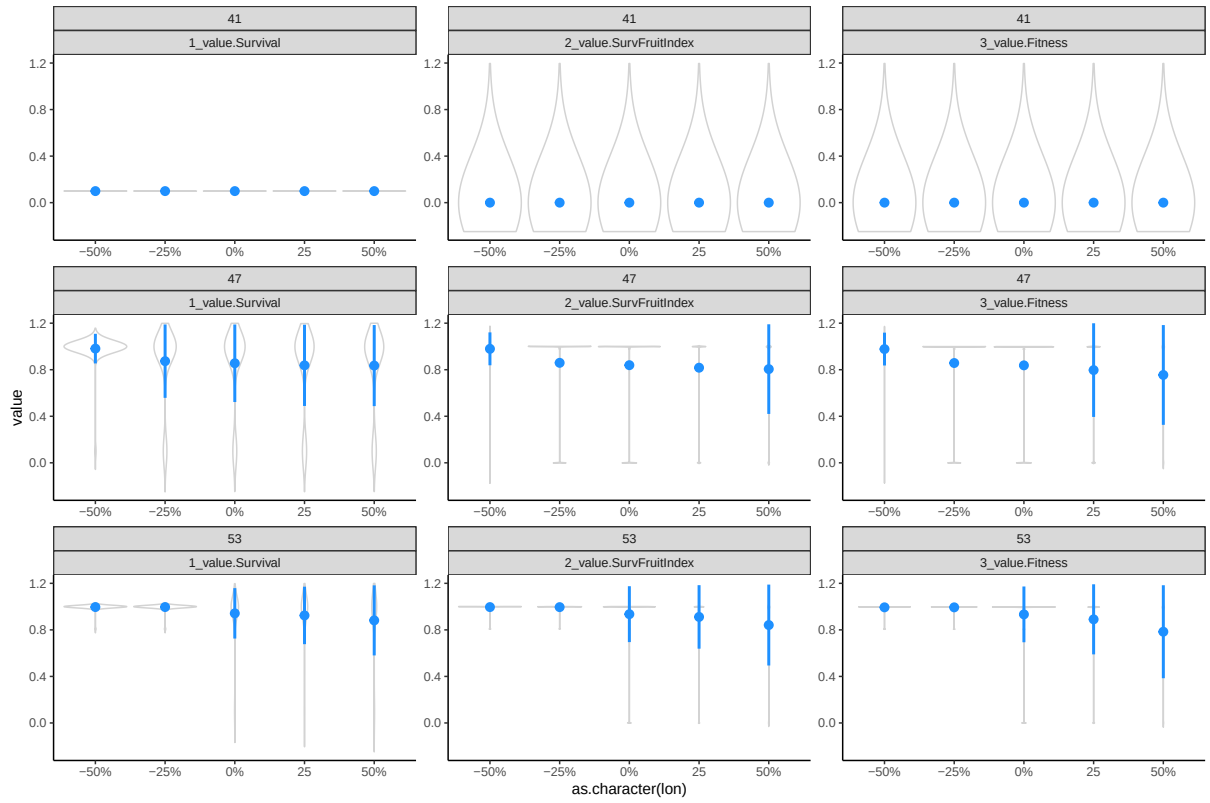
Figure 14: Pinus across changing variance showing three latitudes. There is no survival at low latitudes, while at higher latitudes (see Fig. ??) there is.
