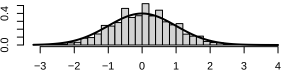
\alpha = 2, \beta = 0.1, t = 1000
