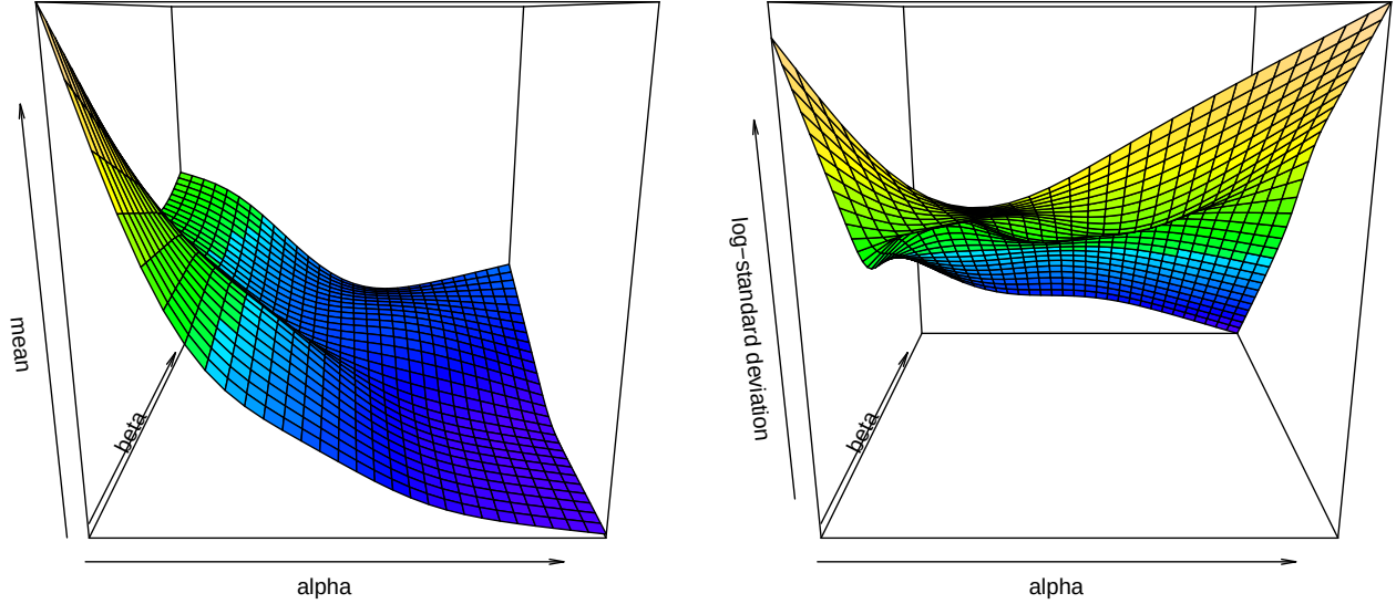
Figure 2: Mean and log standard deviation of lilac-honeysuckle bloom dates ( n = 23,864 from Rosemartin et al. 2015) by baseline temperatures ( \alpha ) and within-season temperature increases ( \beta ) estimated by a generalized additive model. The left figure shows the mean generally decreases at an increasing rate as \alpha and \beta increase. The standard deviation (right figure) can increase or decrease, again depending on the relative values of \alpha and \beta ; for example, see the yellow region corresponds with small \beta and the blue region corresponds with large \beta .
