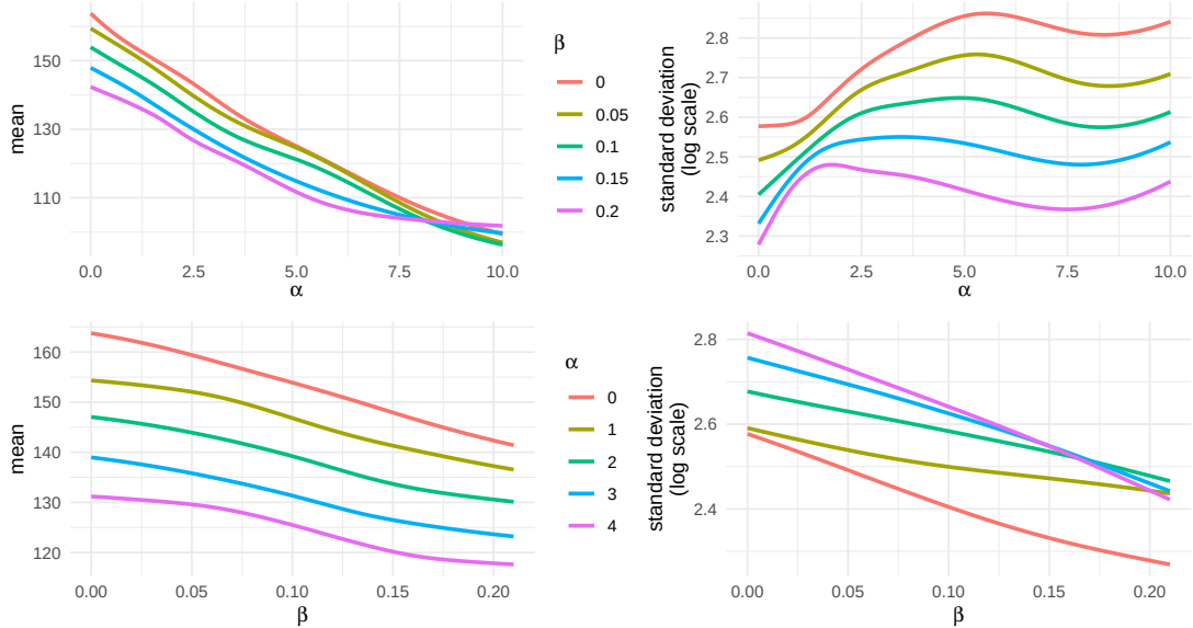
(b) Cross-section plots showing mean (left) and log standard deviation (right) of lilac bloom dates as a function of winter temperature ( \alpha ) holding spring warming ( \beta ) constant (top) and as a function of spring warming ( \beta ) holding winter temperature ( \alpha ) constant (bottom).
