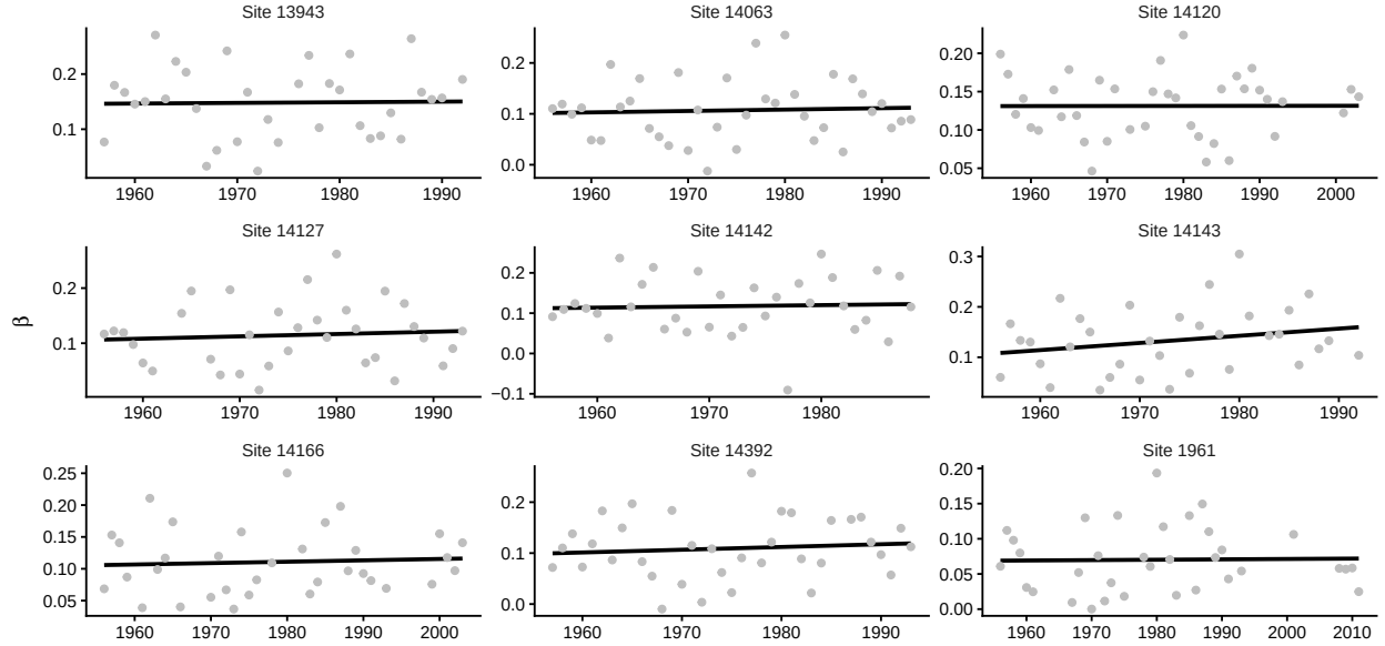
Figure 7: Changes in \beta for the nine sites from lilac-honeysuckle data (Rosemartin et al. 2015) with longest running records as as measured by GHCND stations nearby. Trend line calculated using linear regression.
