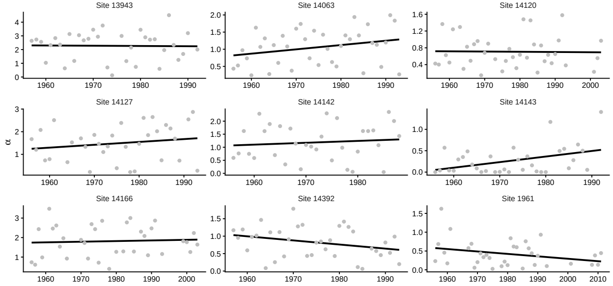
Figure 6: Changes in \alpha for the nine sites from lilac-honeysuckle data (Rosemartin et al. 2015) with longest running records as as measured by GHCND stations nearby. Trend line calculated using linear regression.
