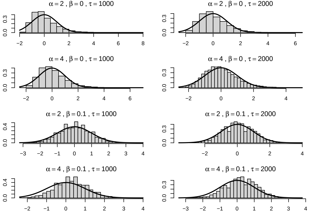
Figure 11: Simulations comparing the distribution of bloom dates (histogram) with an asymptotic approximation (solid line) under two regimes: winter (top two rows) and spring (bottom two rows).
