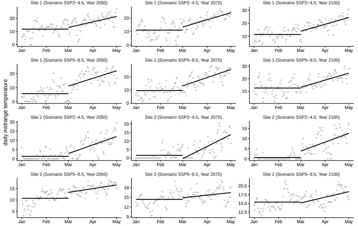
Figure 8: Springtime daily midrange temperatures (points) with \alpha (mean from Jan to Feb) and \beta (slope from Mar to Apr) for two randomly selected sites under two scenarios for the years 2050, 2075, and 2100 from the NEX-GDDP-CMIP6 dataset (Thrasher et al. 2022). Temperatures below 0 are set to 0.
