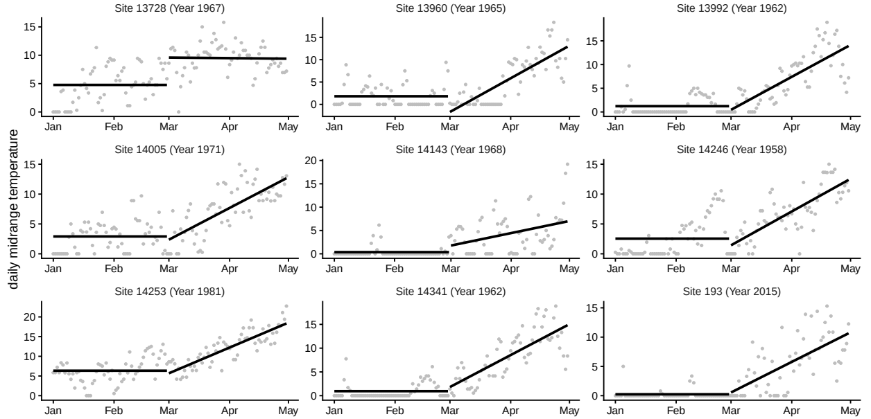
Figure 5: Springtime daily midrange temperatures (points) with \alpha (mean from Jan to Feb) and \beta (slope from Mar to Apr) for nine randomly selected sites from lilac-honeysuckle dataset (Rosemartin et al. 2015) as measured by GHCND stations nearby. Temperatures below 0 are set to 0.
