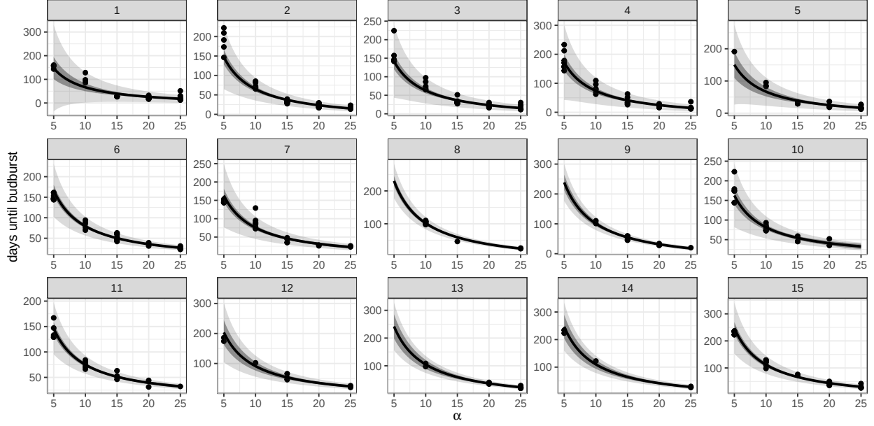
Figure 3: Mean time until budburst as a function of the average daily temperature ( \alpha ) in a controlled experiment conducted by Charrier et al. (2011) in which 385 buds were observed on stems sampled from 15 walnut trees ( Juglans regia and Juglans regia \times nigra hybrids) trees, chilled at 4°C, and then warmed in different temperatures environments (x-axis) with the same photoperiod conditions across temperatures until budburst. For each tree (panel), we show the observed dates (points), fitted mean (solid line), 95% confidence interval (inner grey region, approximately two standard errors), and 95% prediction interval (outer grey region, approximately two standard deviations). The figure shows that the mean and variance are nonlinear functions of temperature even when biological factors such as chilling and photoperiod are held fixed. Both decrease with increasing temperatures as predicted by the thermal-sum model.
