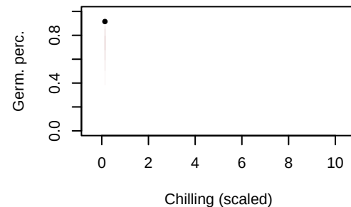
Eucalyptus delegatensis , Prov: 1, Time: -0.44
