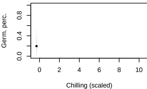
Eucalyptus_delegatensis, Prov: 2, Time: -0.43
