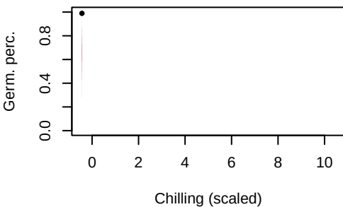
Maackia_taiwanensis, Prov: 18, Time: 0.88
