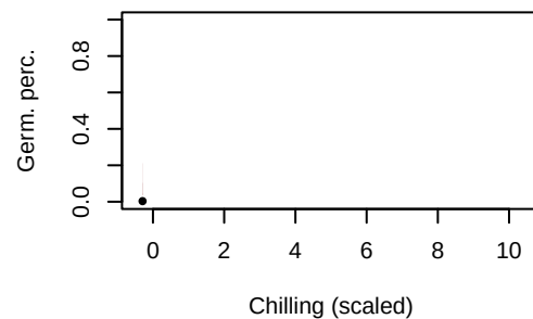
Eucalyptus_delegatensis, Prov: 2, Time: -0.47
