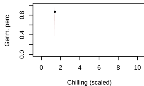
Maackia_taiwanensis, Prov: 19, Time: 2
