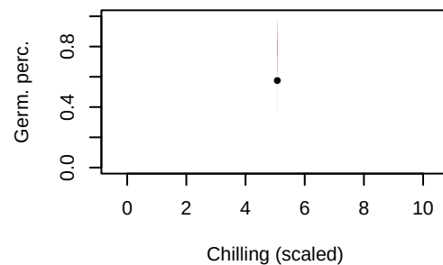
Maackia_taiwanensis, Prov: 19, Time: 3.19
