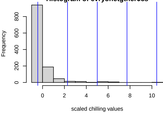
Histogram of evryonetgther$cs
