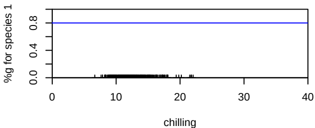
%g-Chilling Sensitivity for species 1
