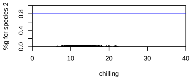
%g-Chilling Sensitivity for species 2
