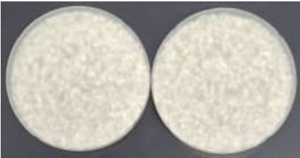
Trichophyton rubrum Control
