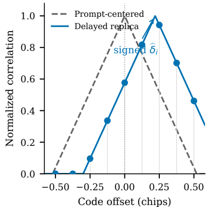
(a) Nine-tap delay sensor
