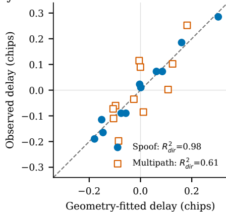
(c) One displacement explains spoof delays
