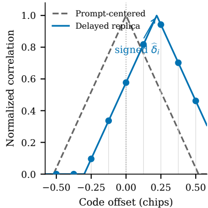
(a) Nine-tap signed-delay sensor
