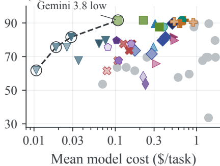
(b) OSWorld: cost
