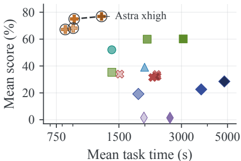
(c) OSWorld2: time
