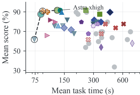
(a) OSWorld: time
