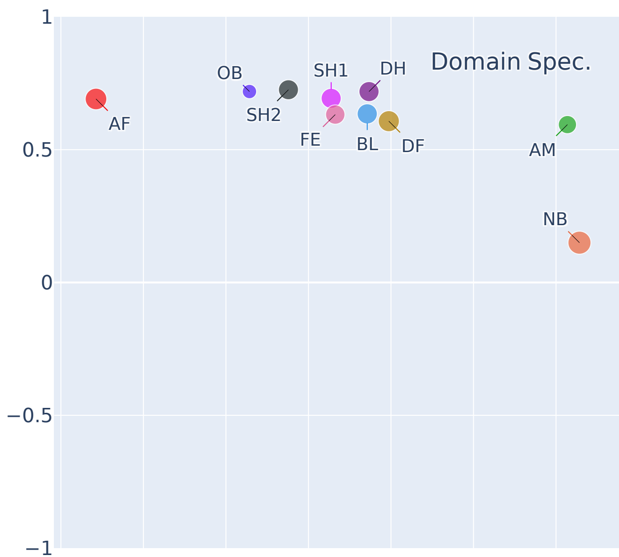
Correlation
