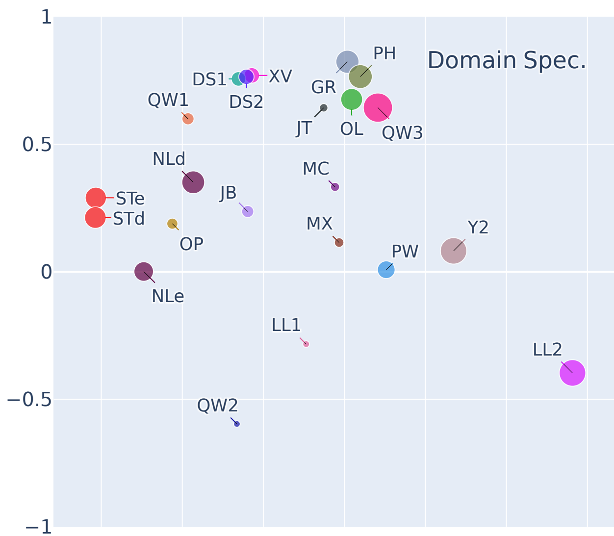
Correlation
