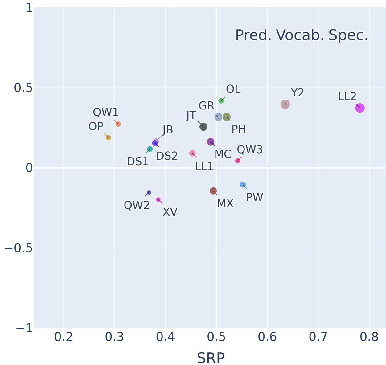
Correlation
