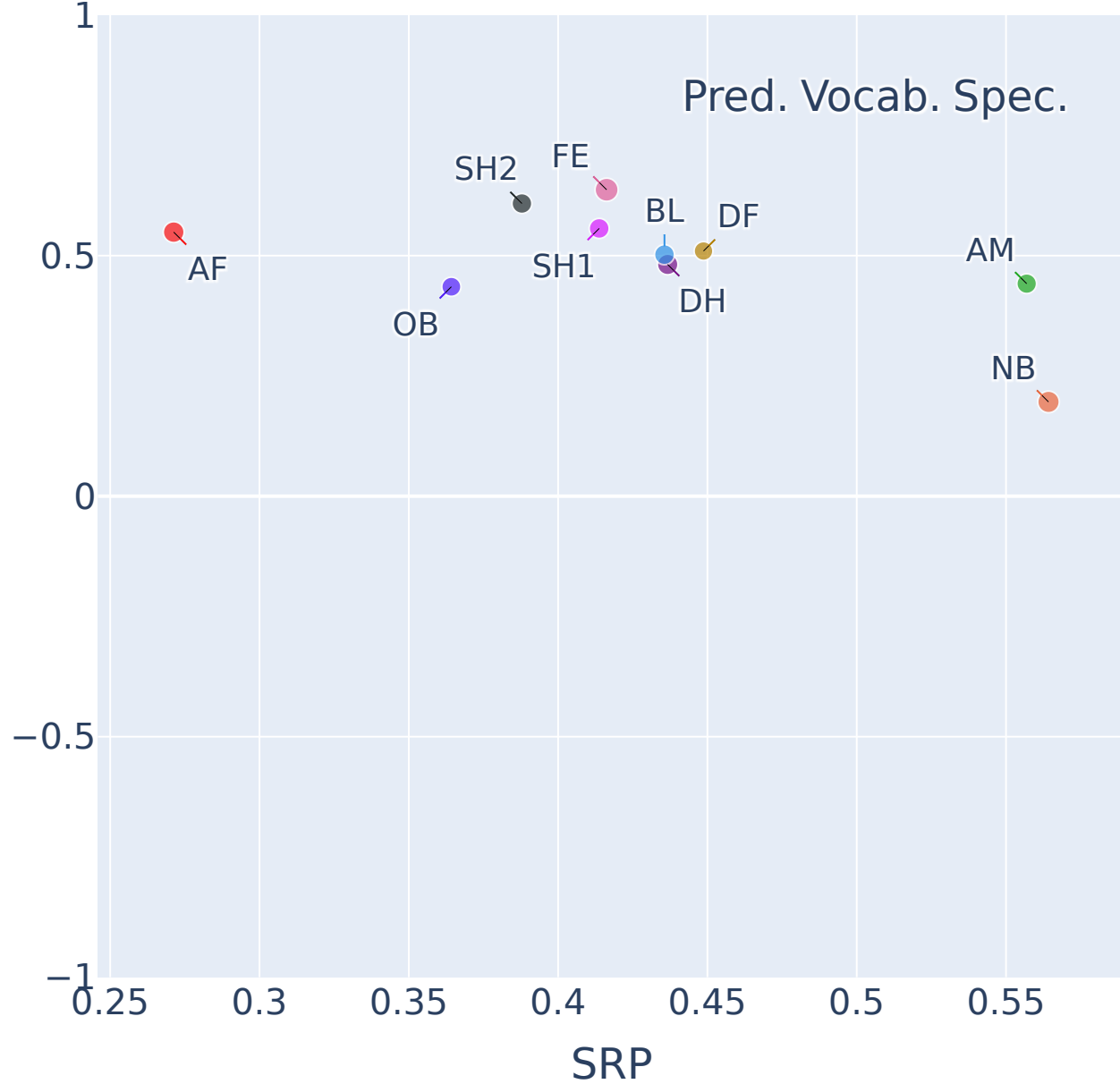
Correlation
