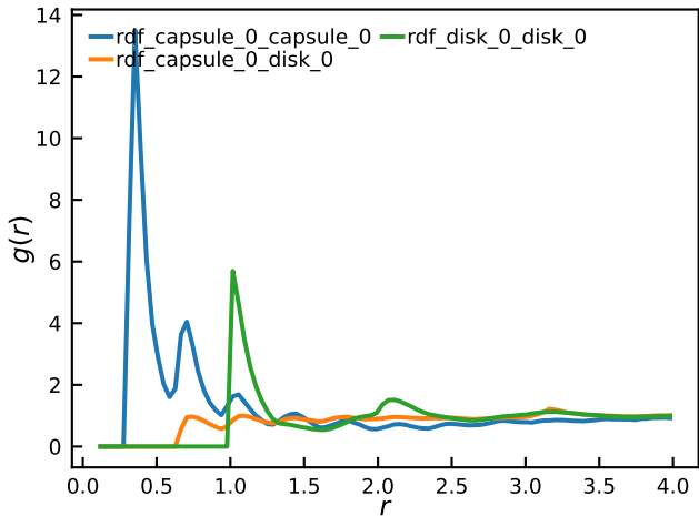
Radial Distribution Function
