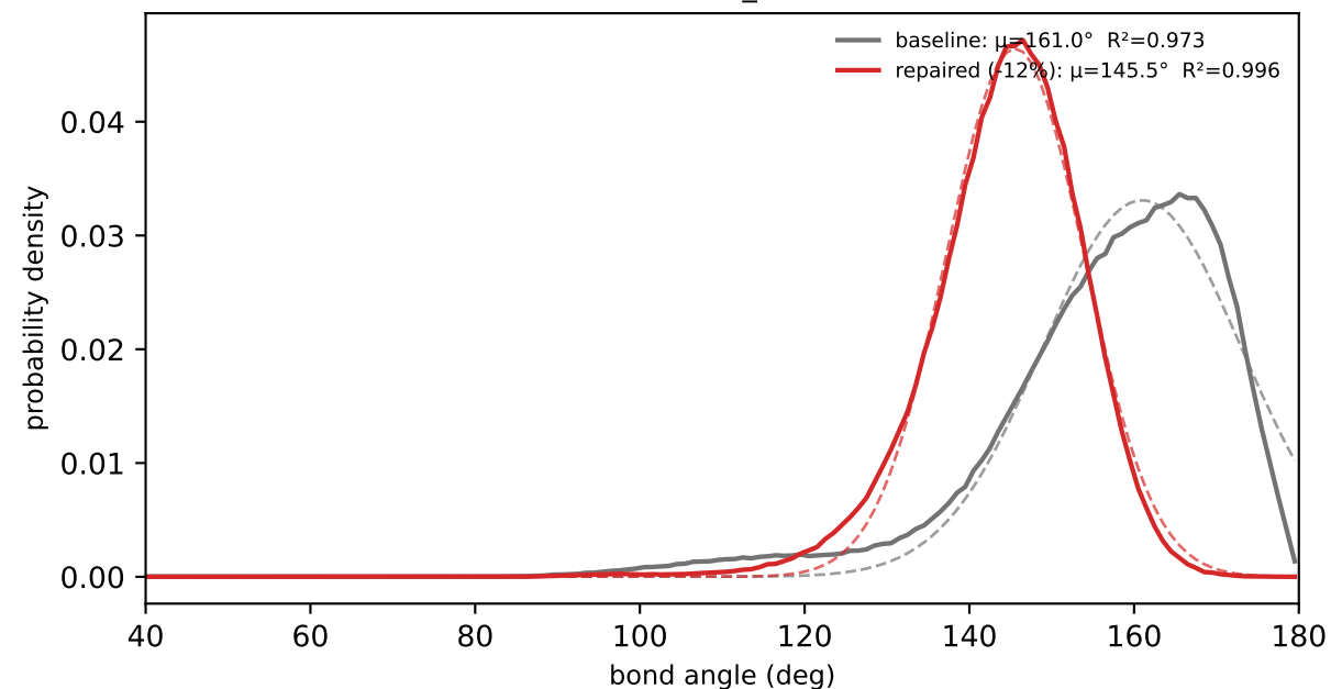
SC1-SC1-SC1 (n_obs=450018)
