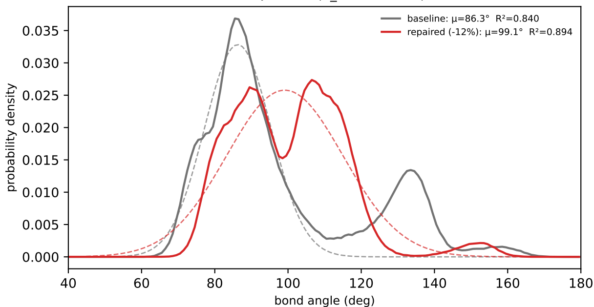
SC1-SC1-TN5a (n_obs=950038)
