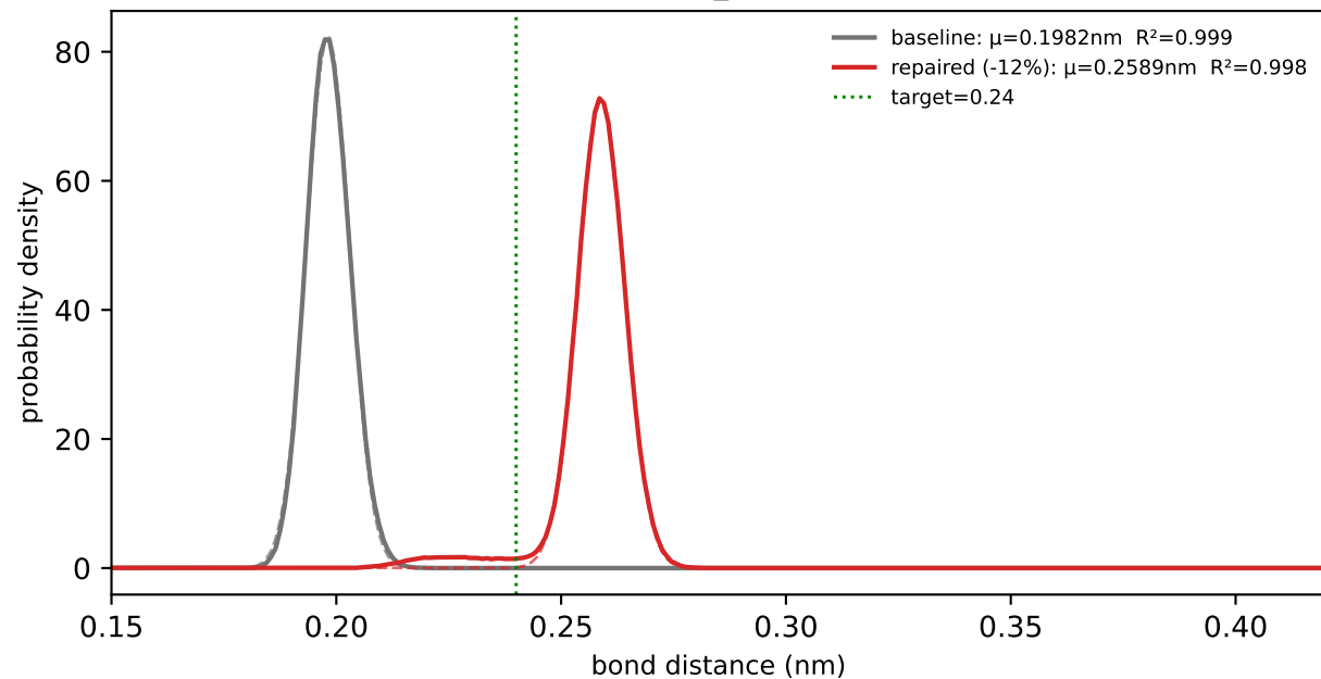
SC1-SC1 (n_obs=475019)
