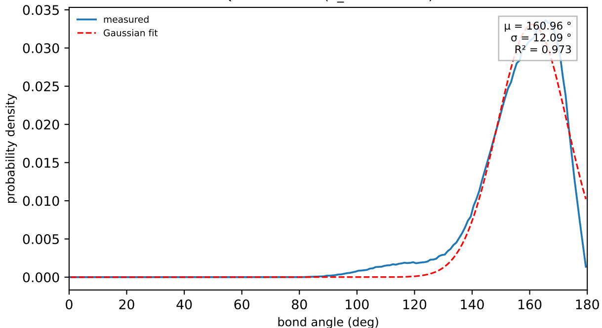
SC1-SC1-SC1 (n_obs=450018)
