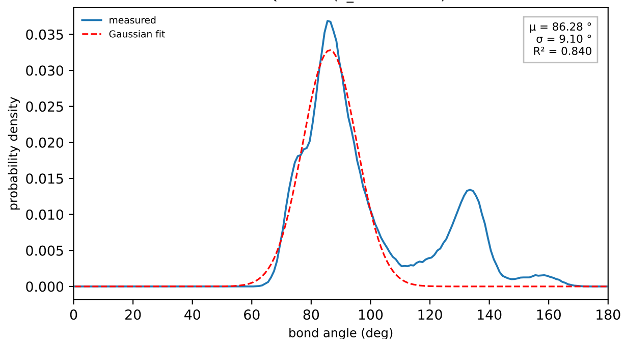
SC1-SC1-TN5a (n_obs=950038)
