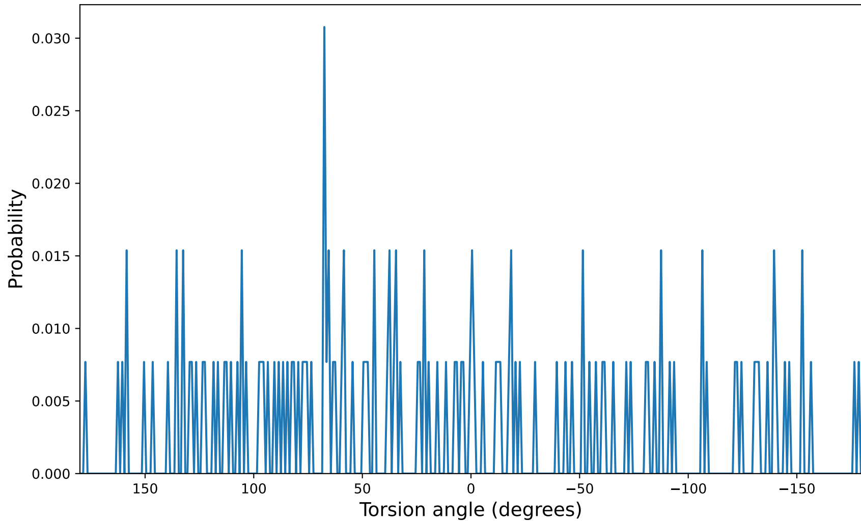
torsion type 1
