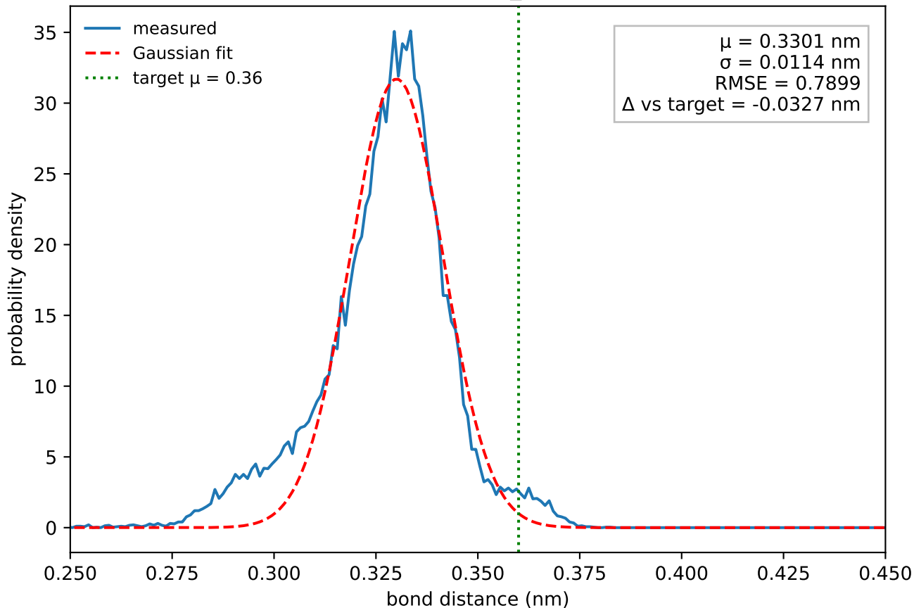
bond distribution (n_obs = 30000)
