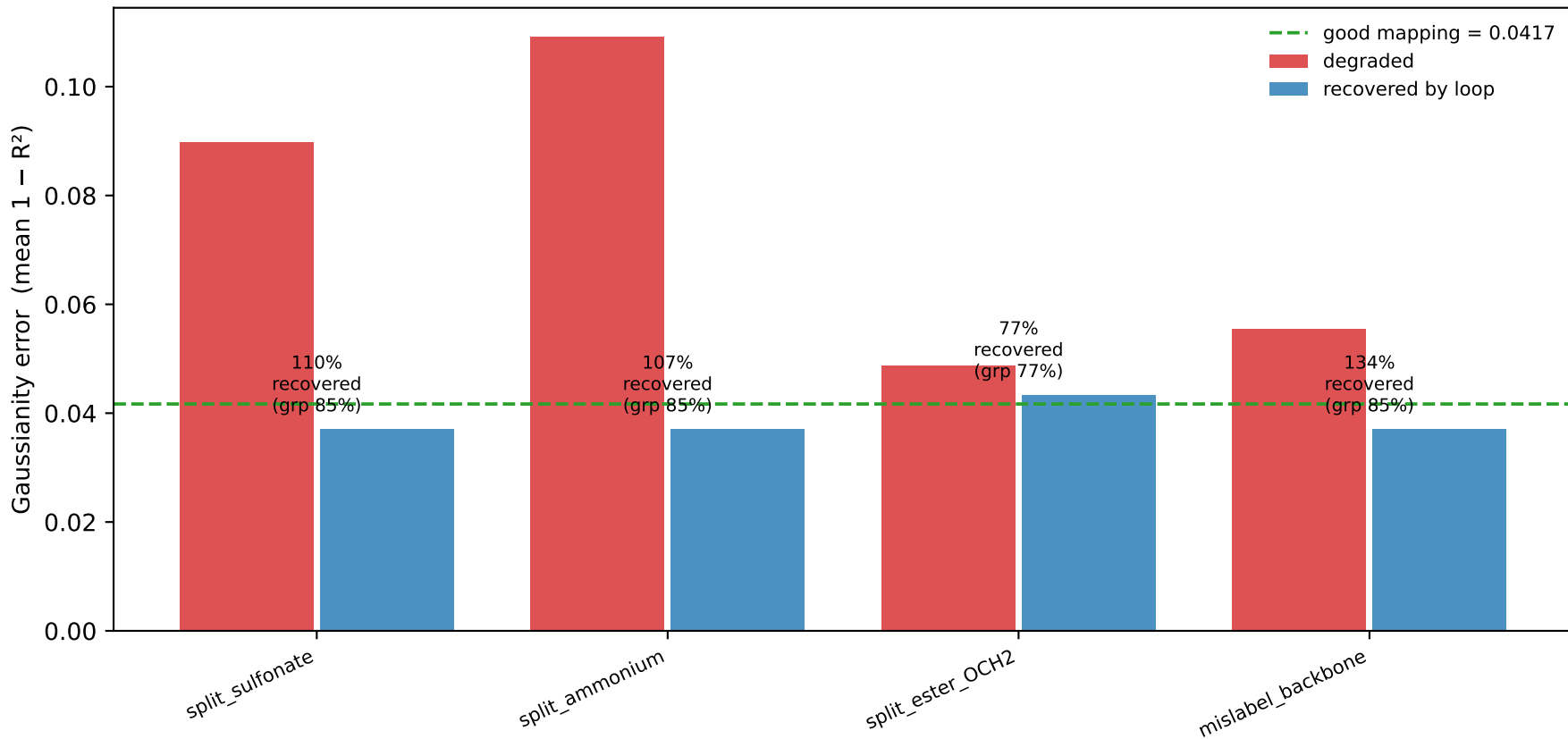
Recover validation — the agent climbs damaged mappings back toward good
