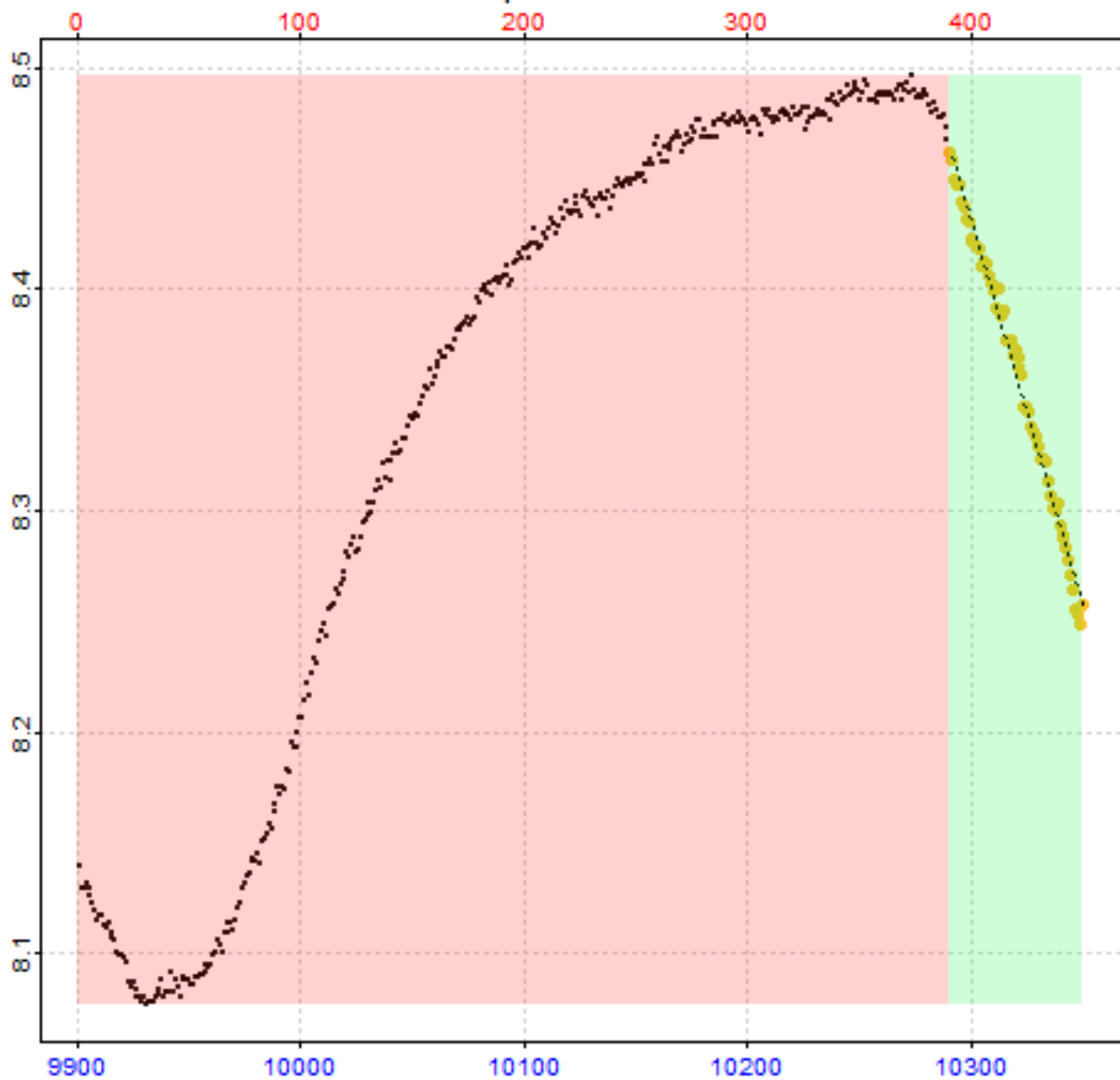
Replicate 23 of 64
