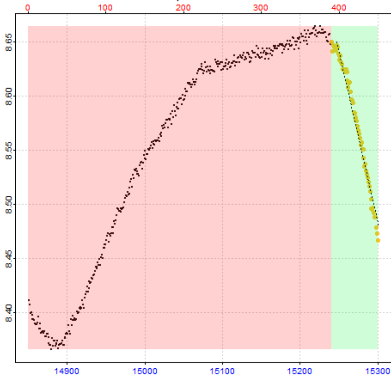
Replicate 34 of 64
