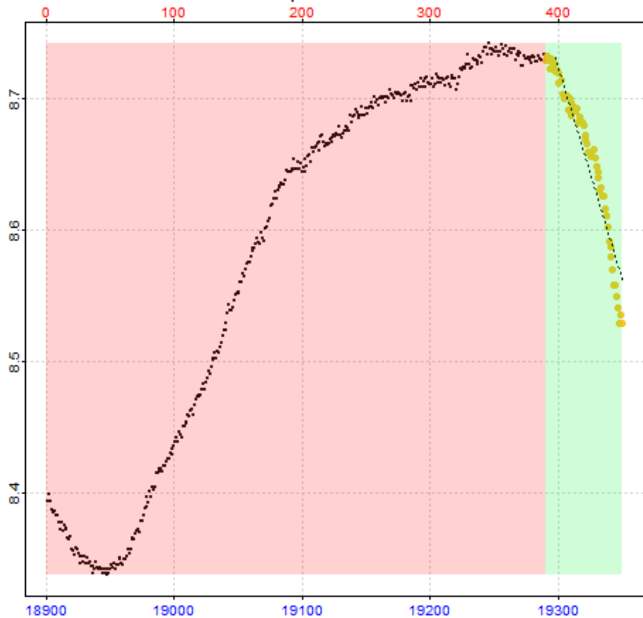
Replicate 43 of 64
