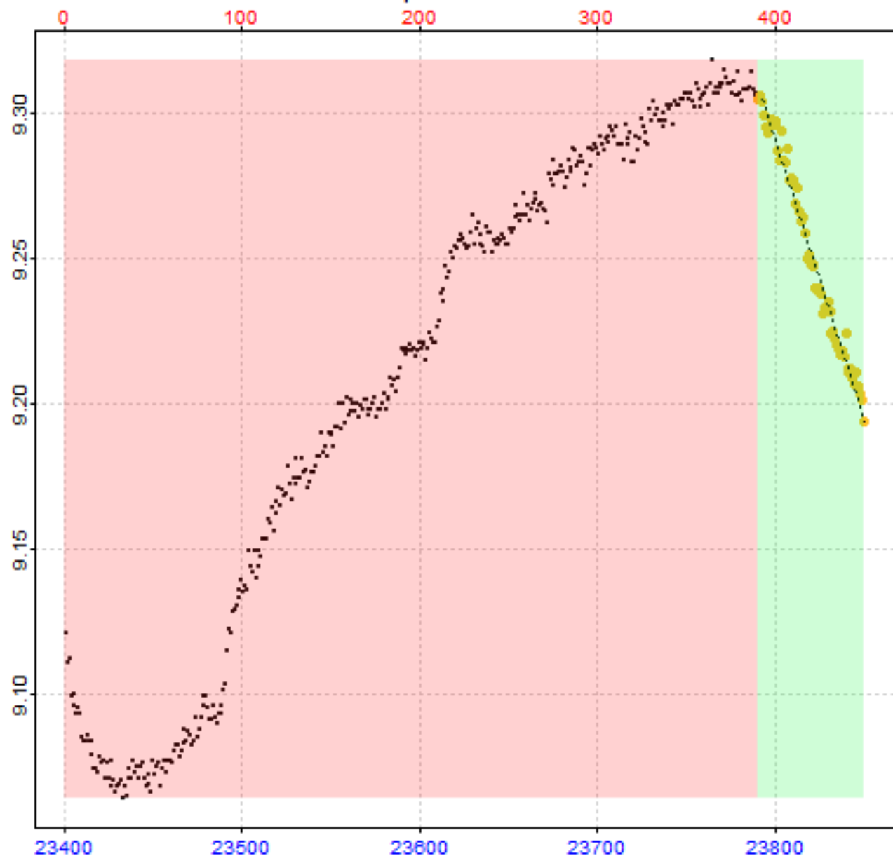
Replicate 53 of 64
