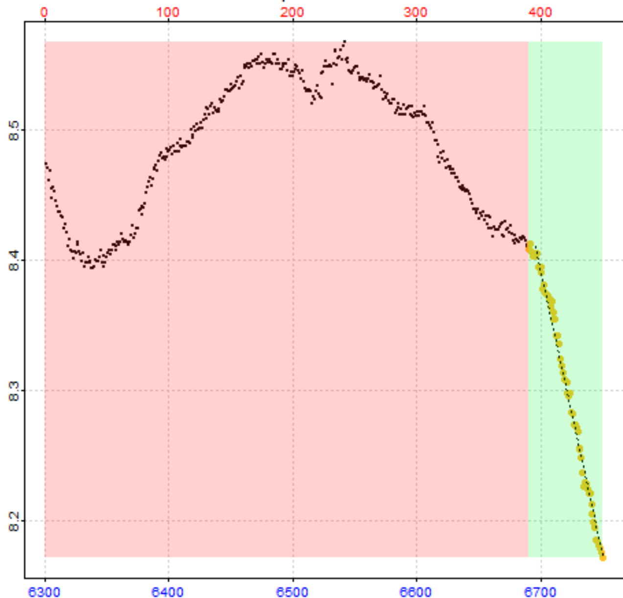
Replicate 15 of 64
