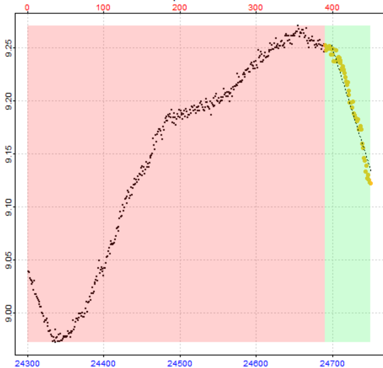
Replicate 55 of 64
