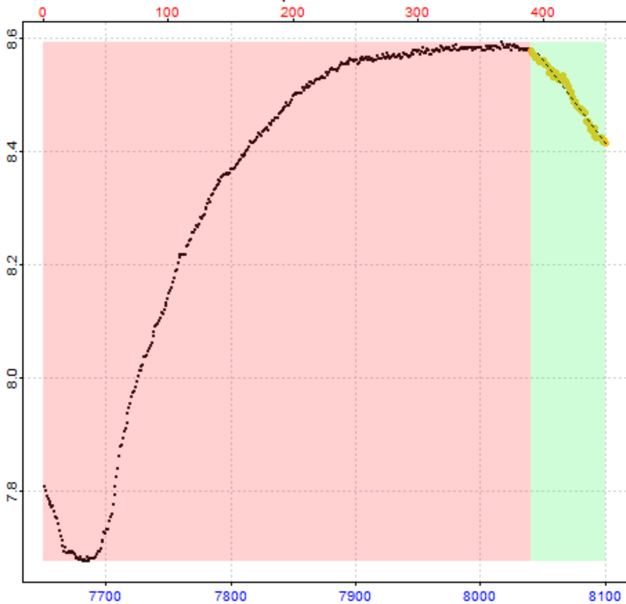
Replicate 18 of 64
