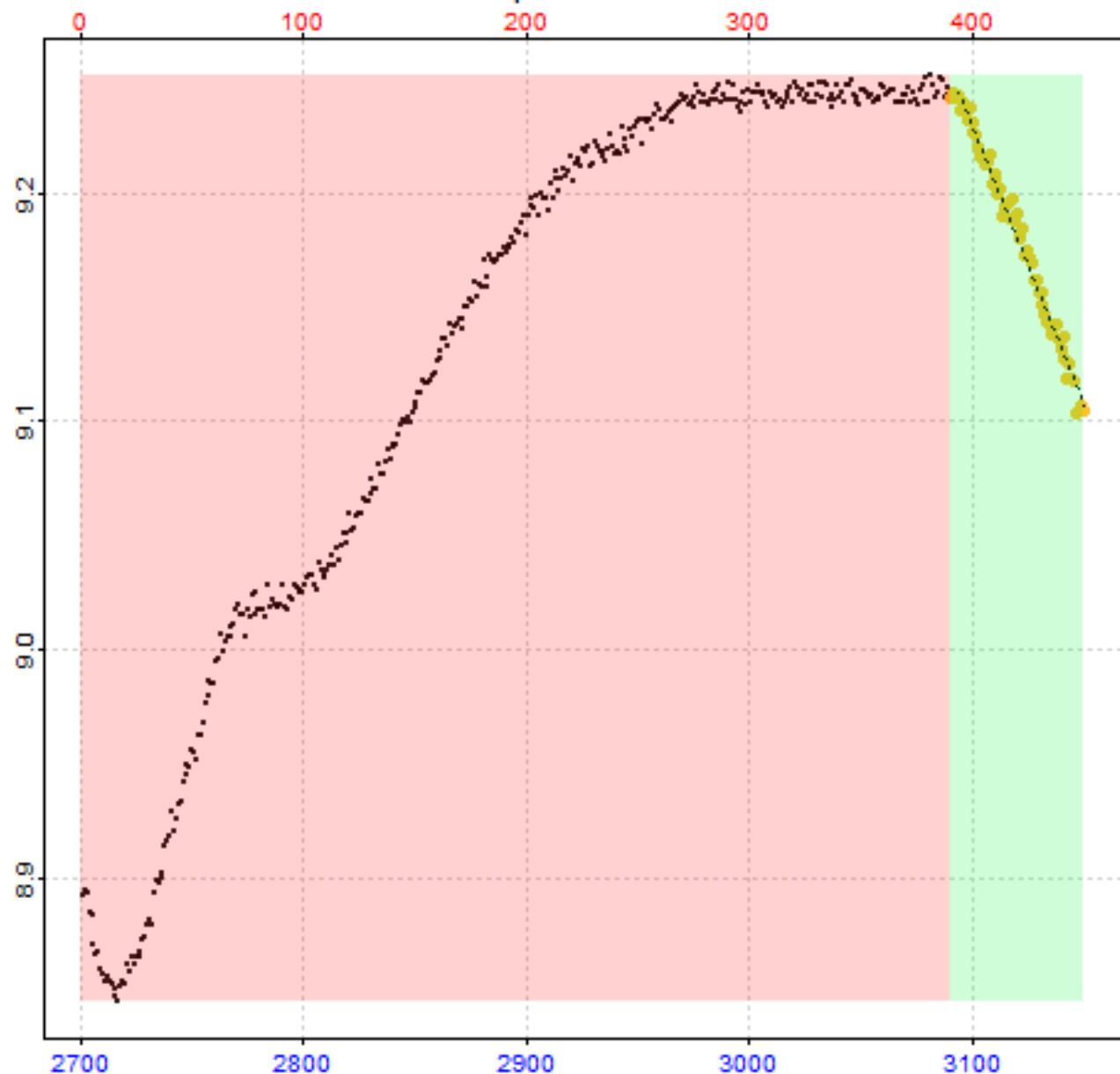
Replicate 7 of 64
