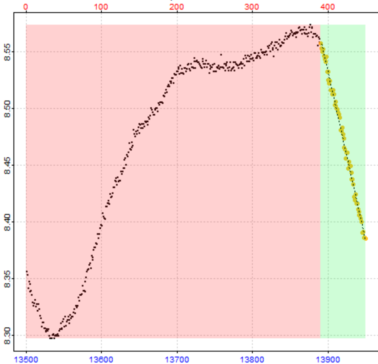
Replicate 31 of 64
