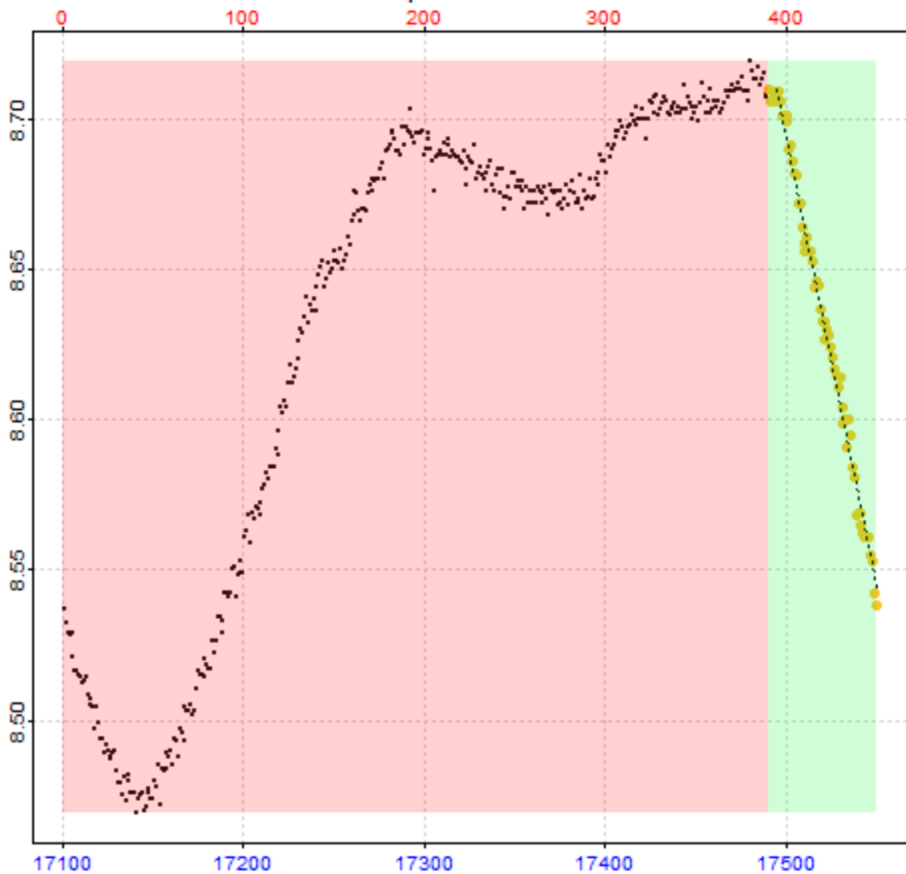
Replicate 39 of 64
