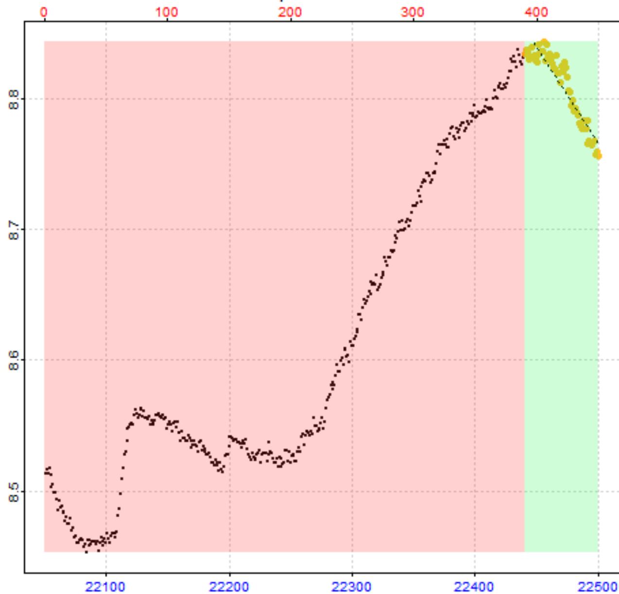
Replicate 50 of 64
