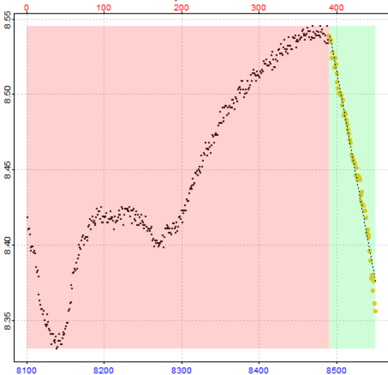
Replicate 19 of 64
