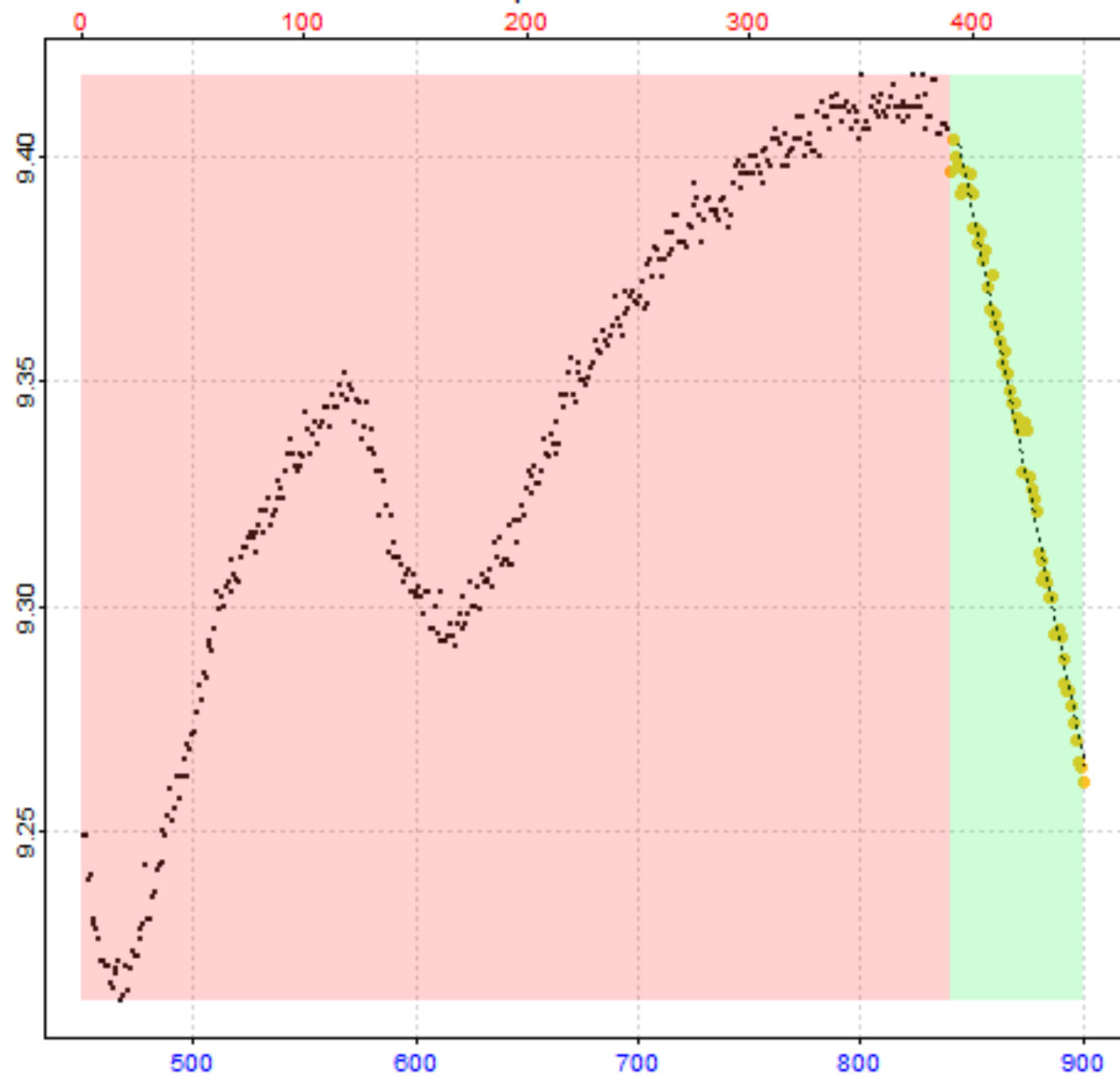
Replicate 2 of 64
