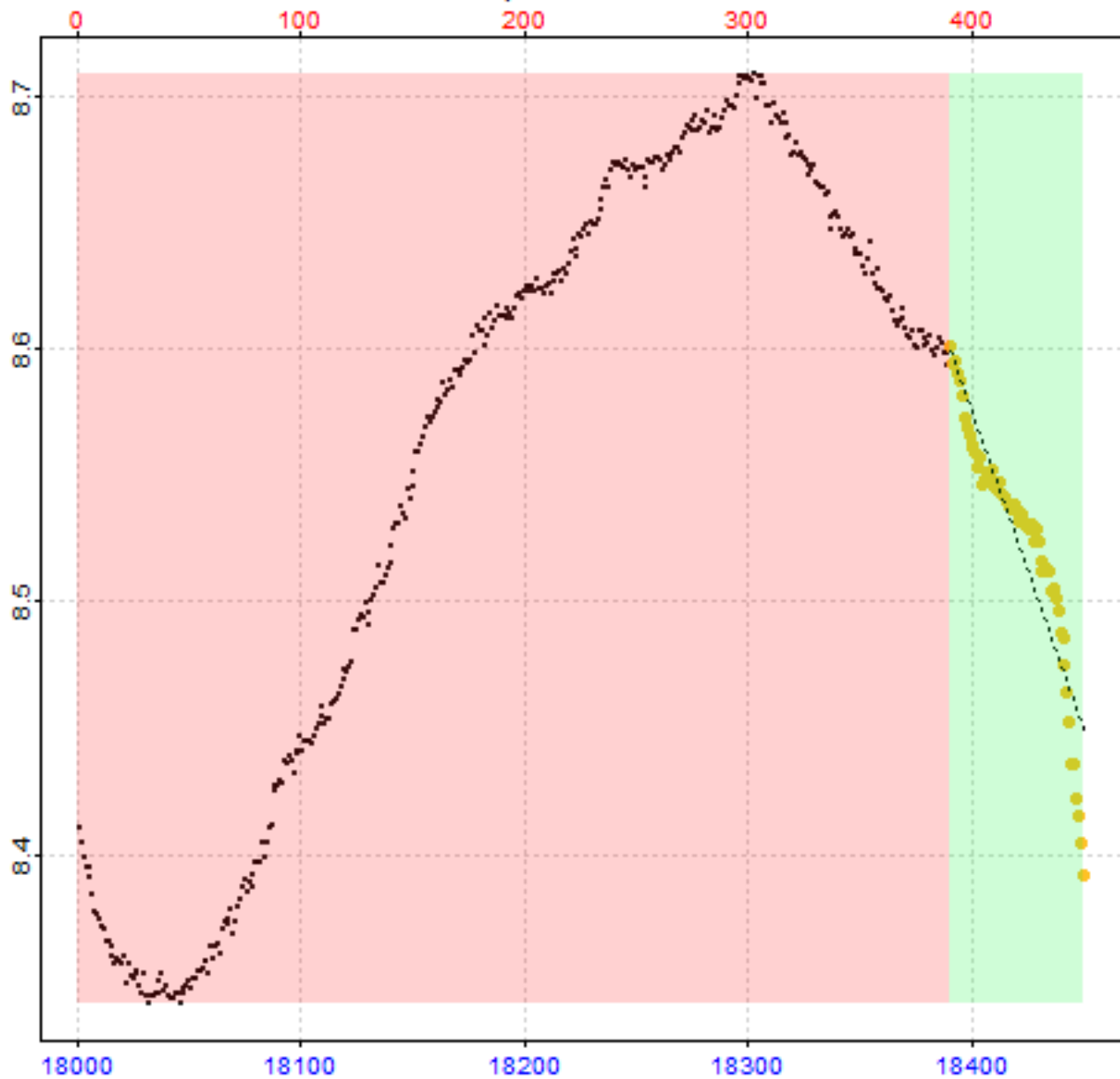
Replicate 41 of 64
