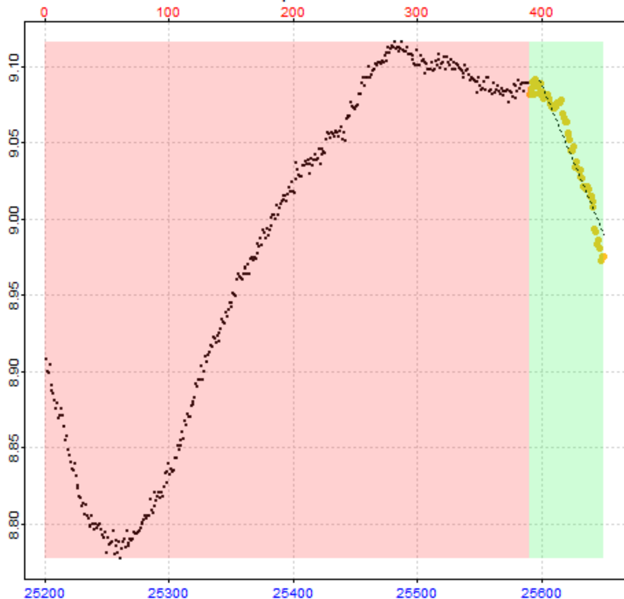
Replicate 57 of 64
