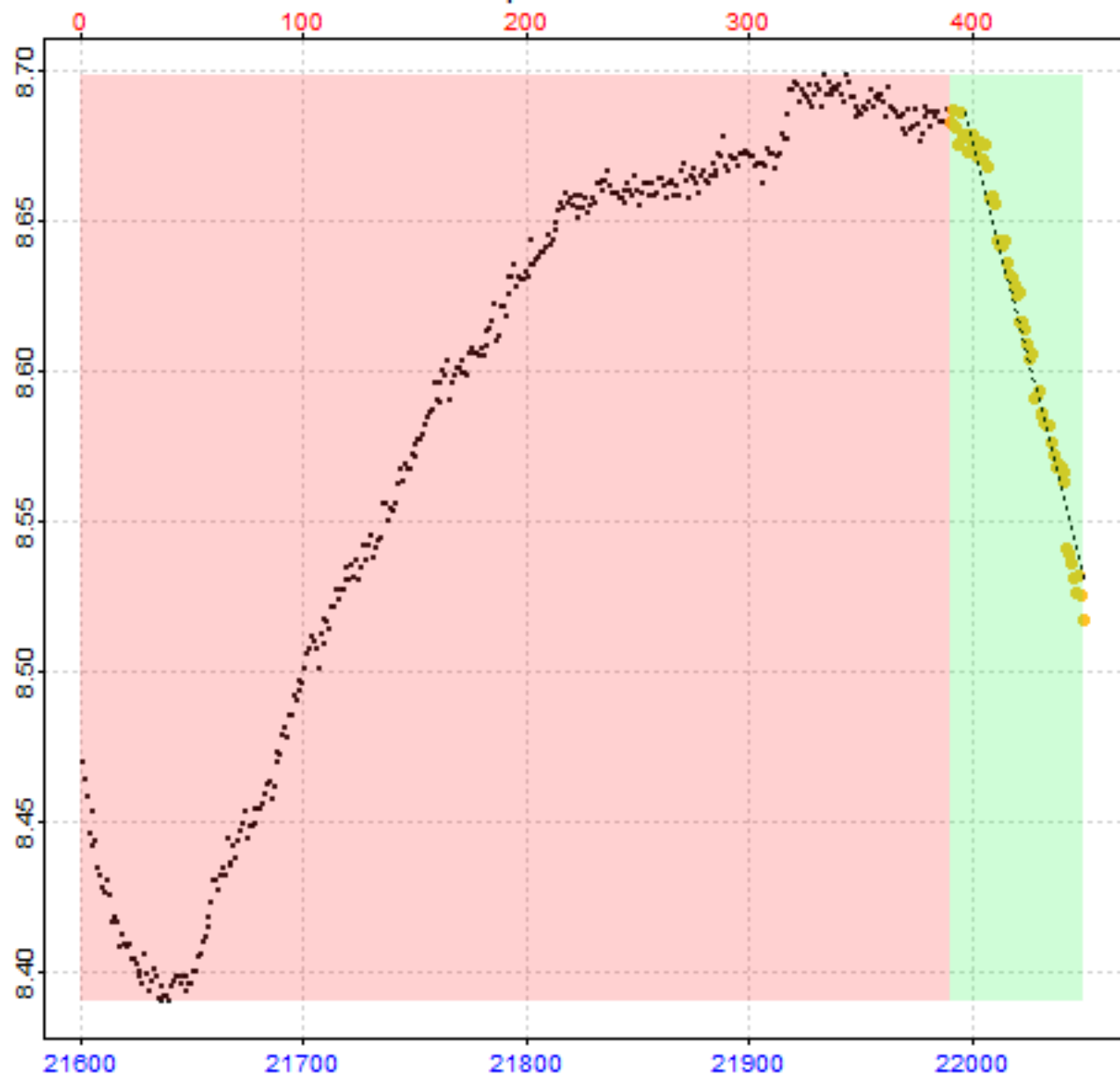
Replicate 49 of 64
