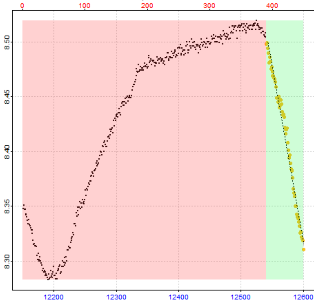
Replicate 28 of 64
