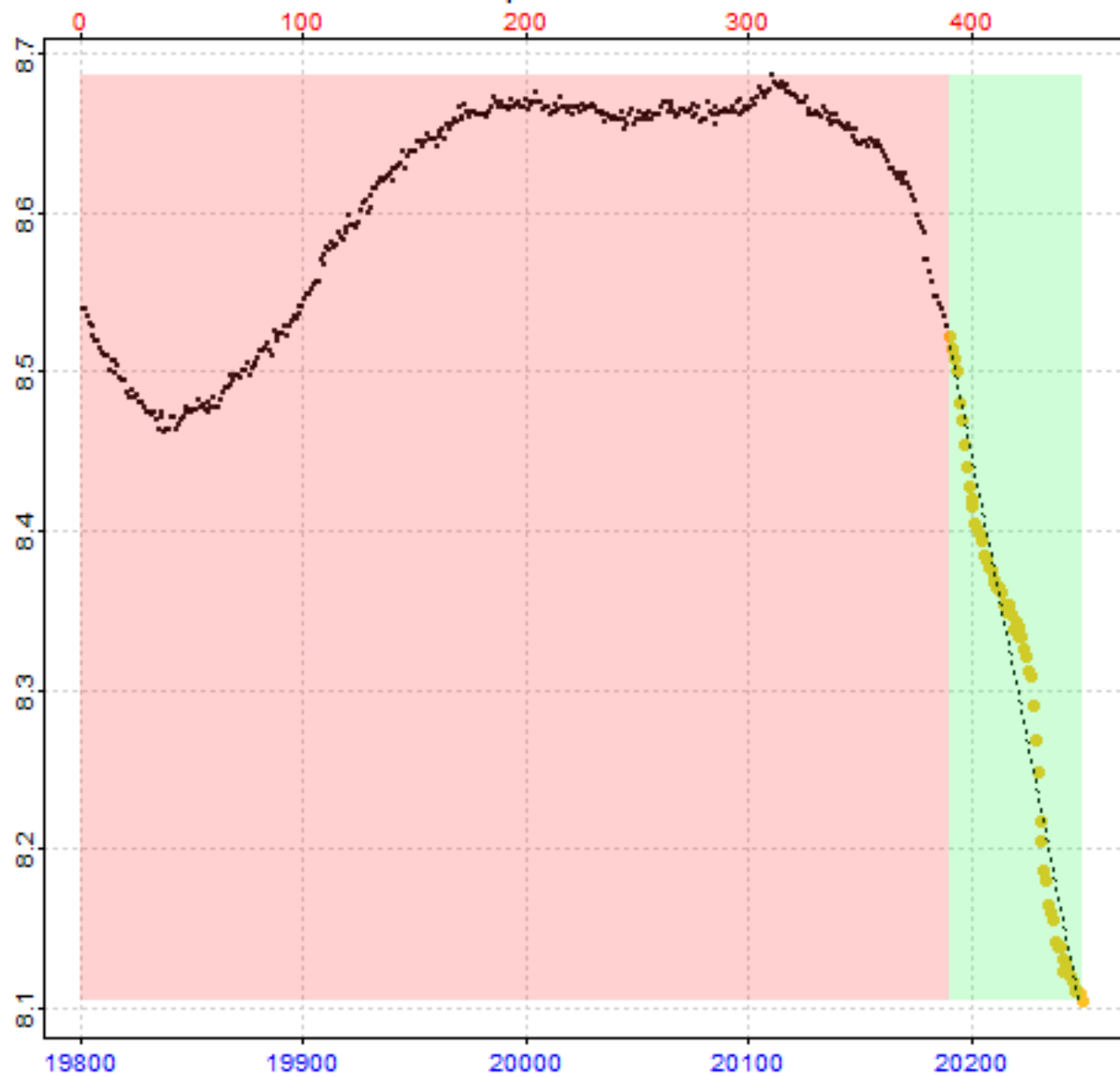
Replicate 45 of 64
