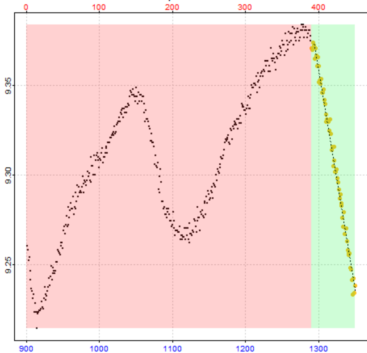
Replicate 3 of 64
