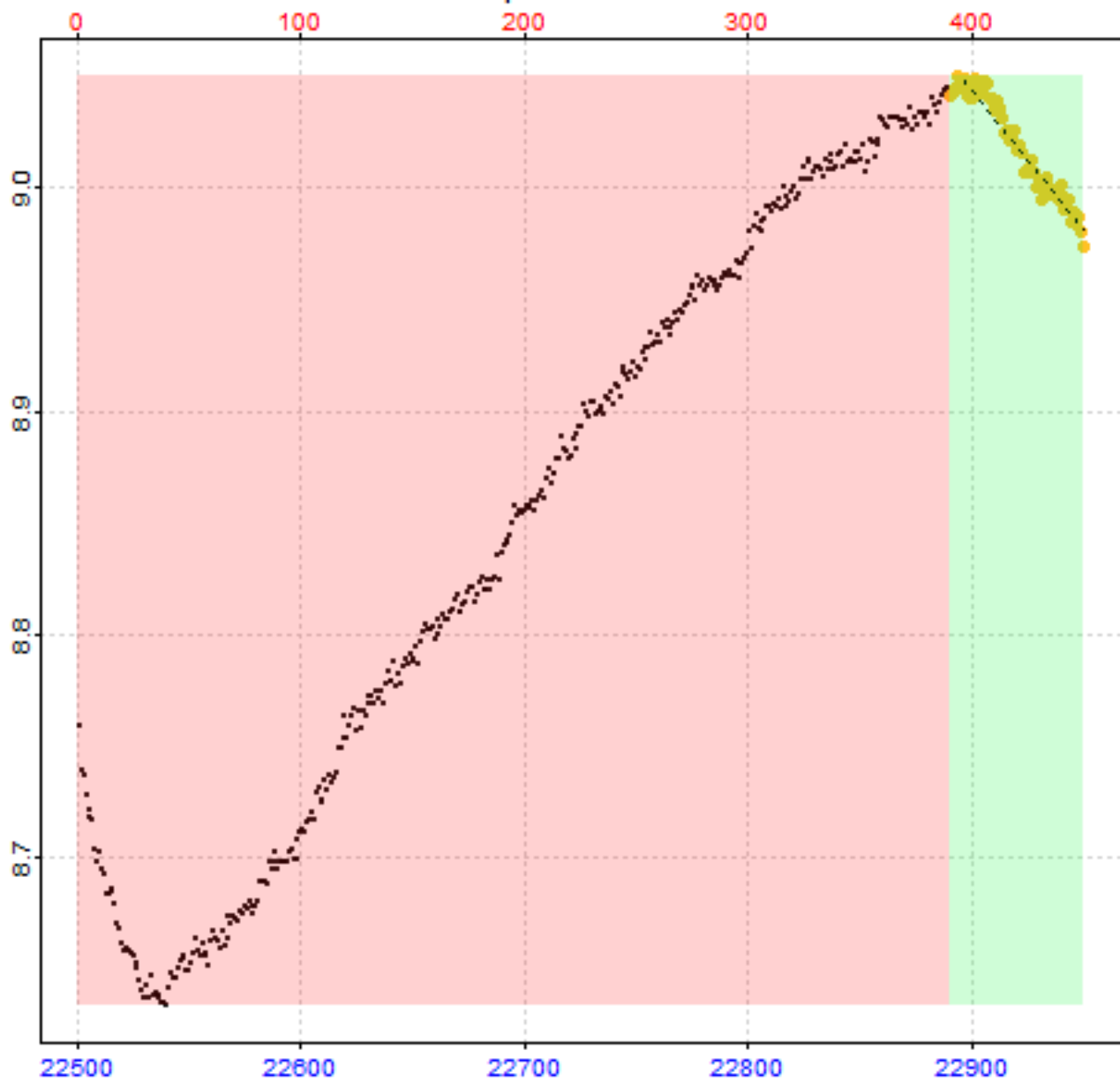
Replicate 51 of 64
