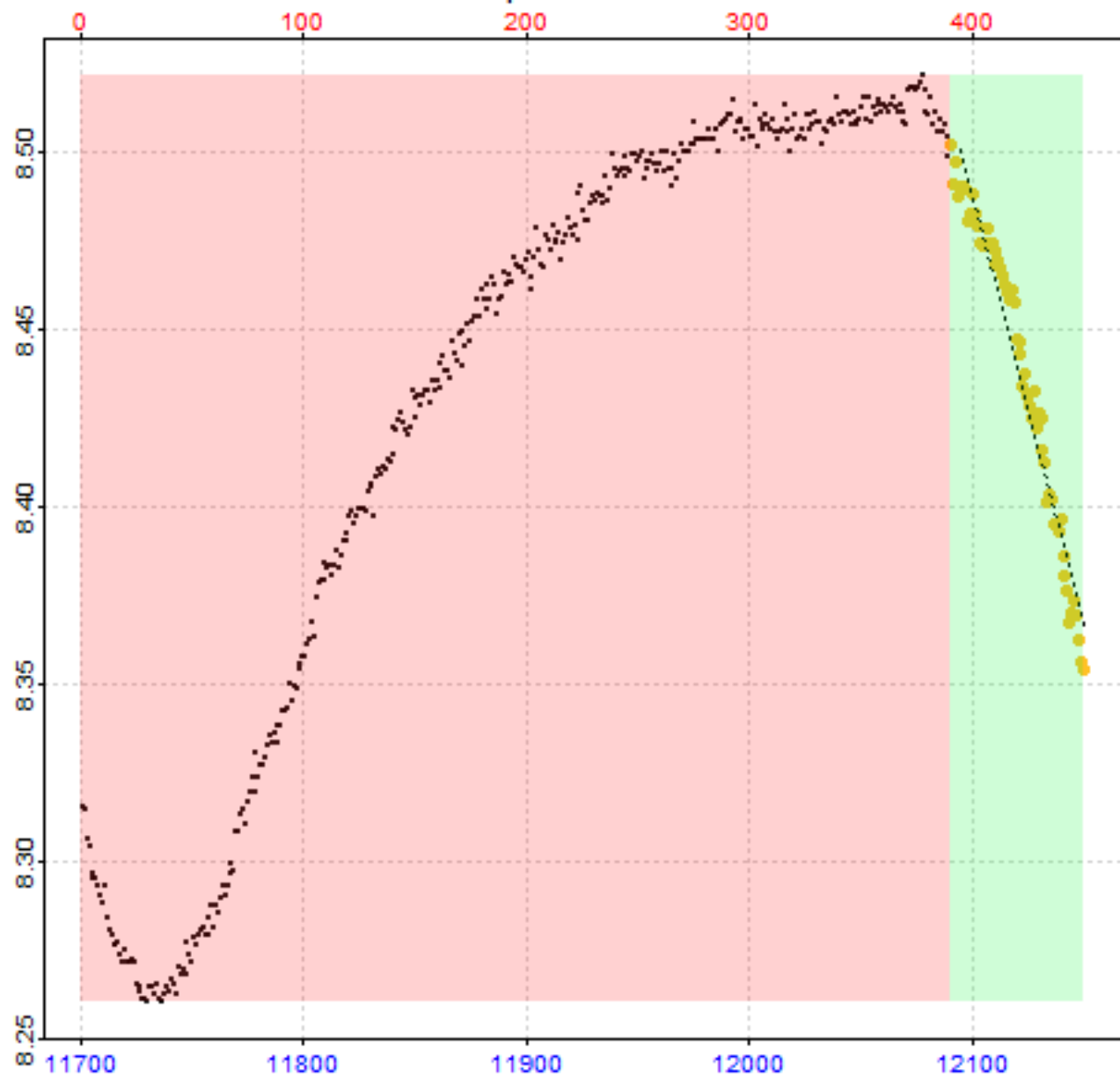
Replicate 27 of 64
