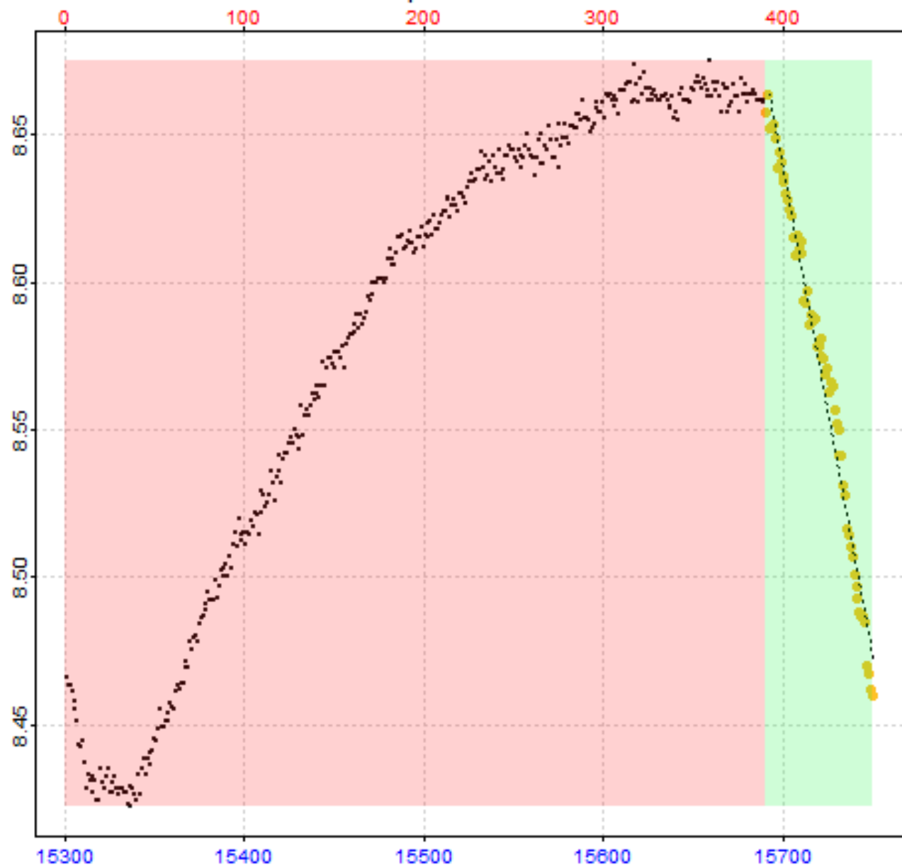
Replicate 35 of 64
