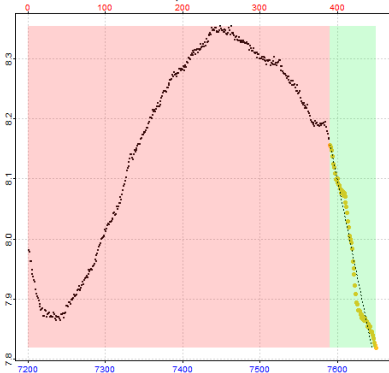
Replicate 17 of 64
