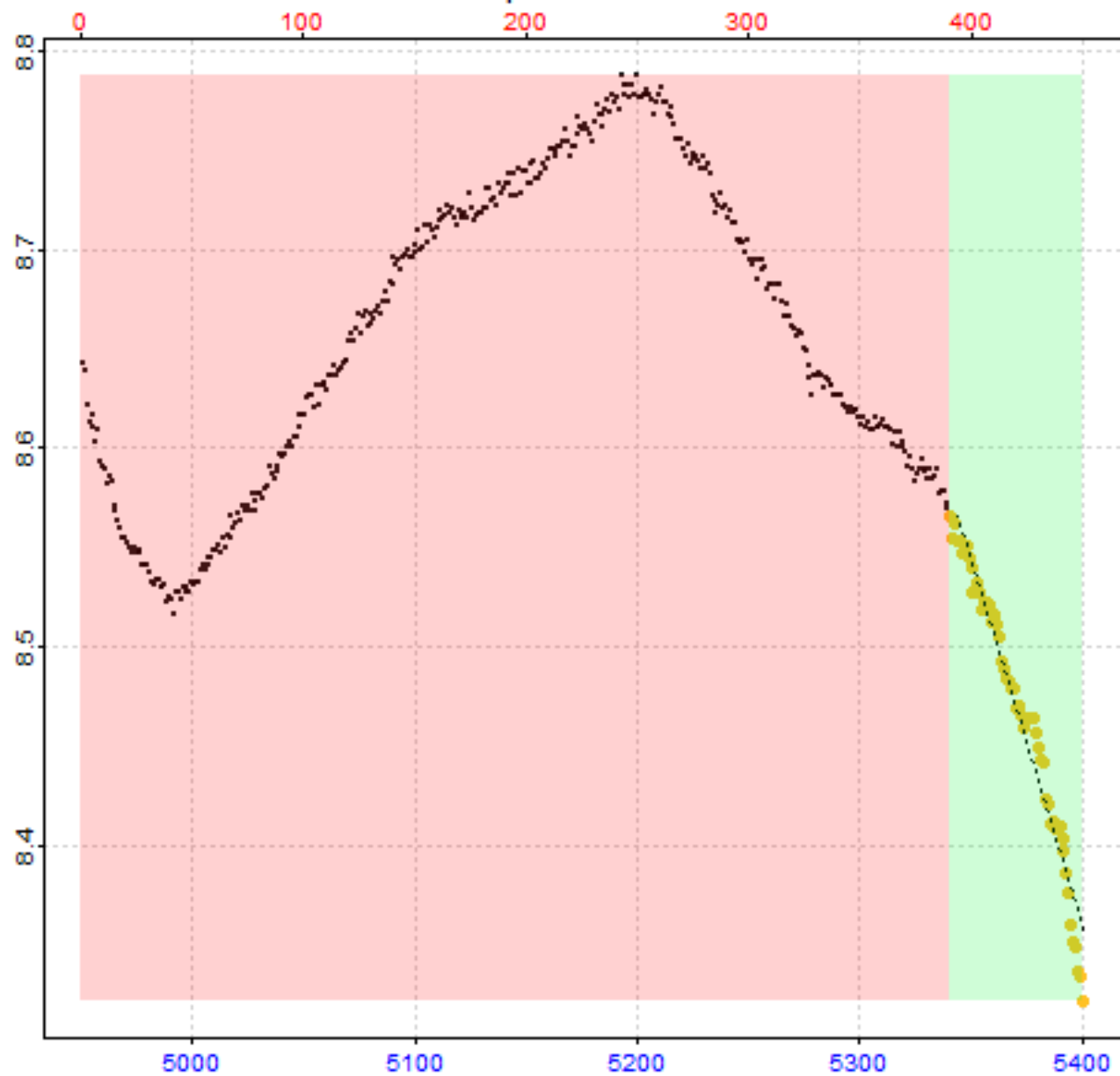
Replicate 12 of 64
