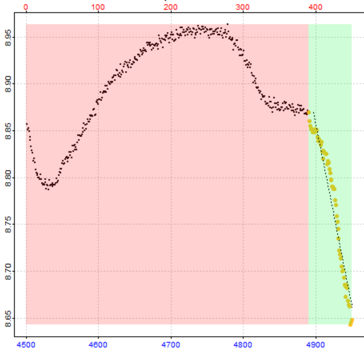
Replicate 11 of 64
