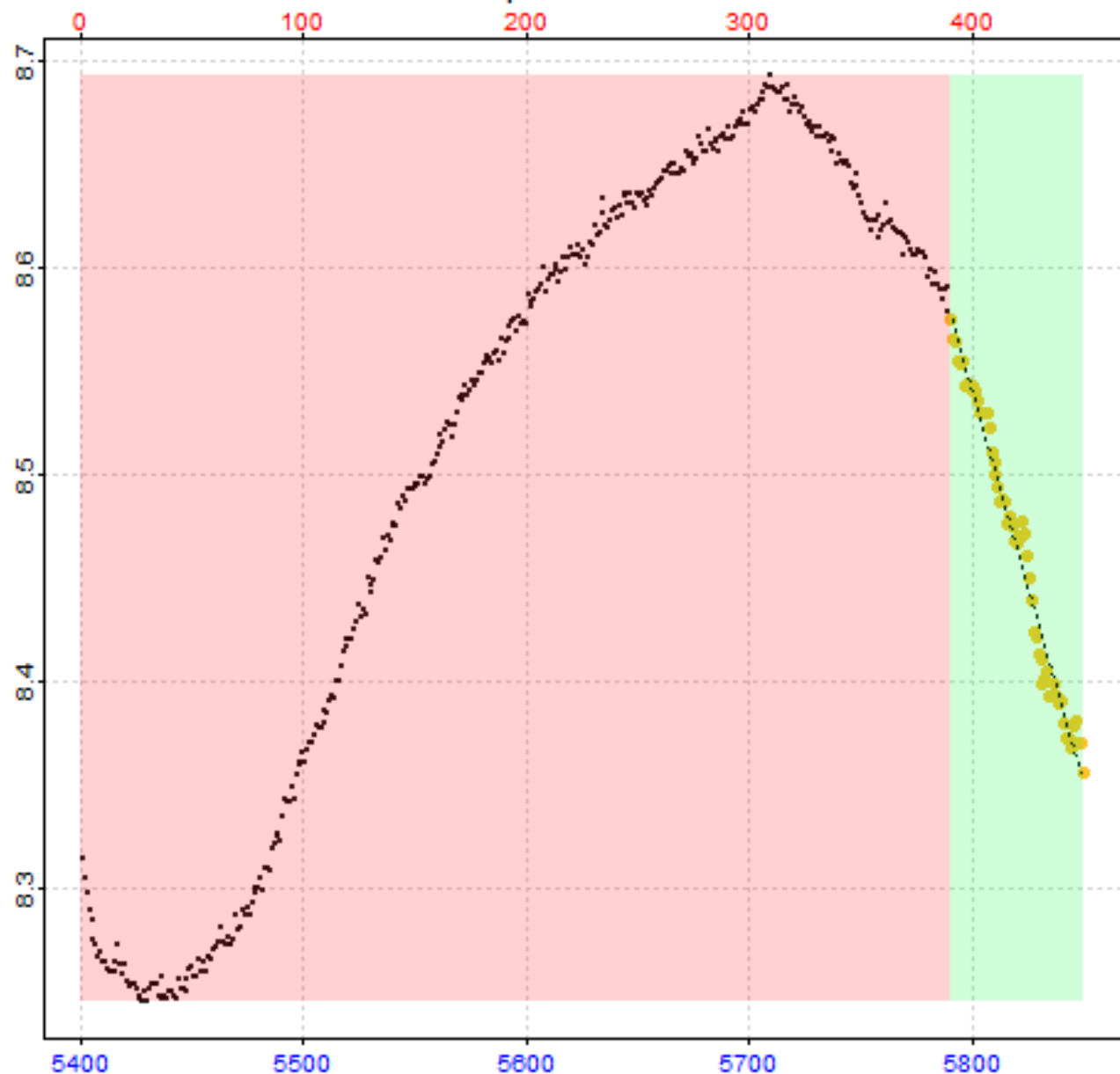
Replicate 13 of 64
