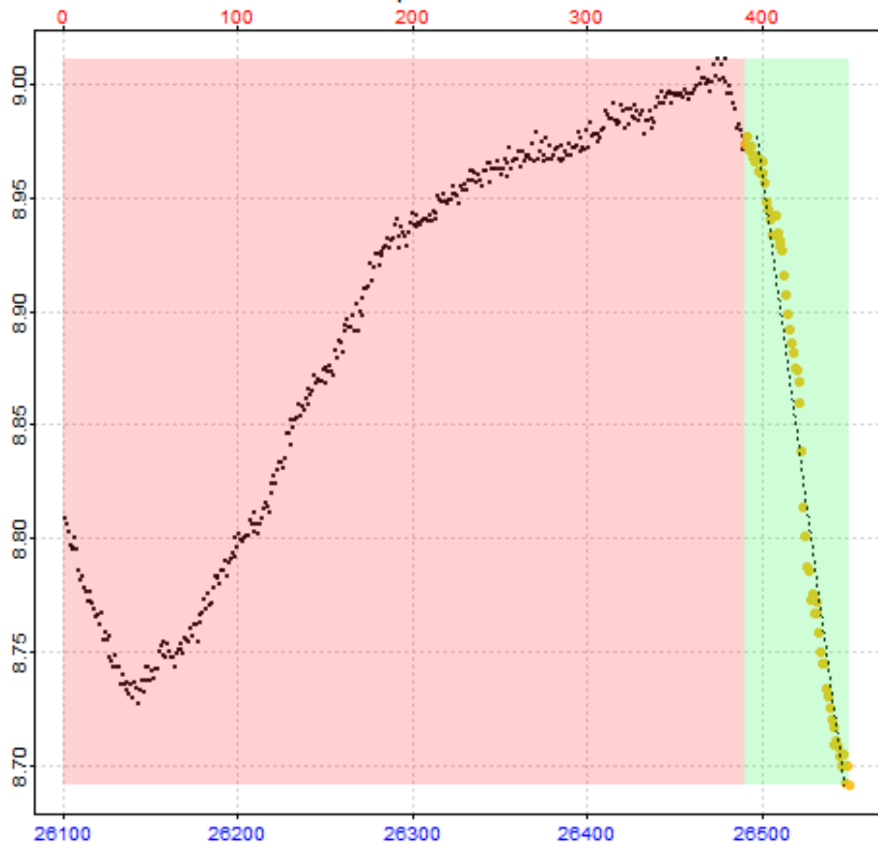
Replicate 59 of 64
