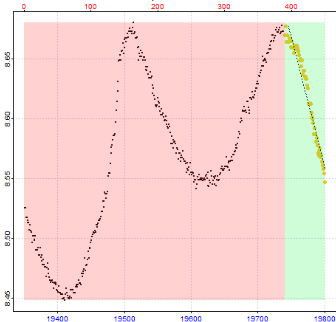
Replicate 44 of 64
