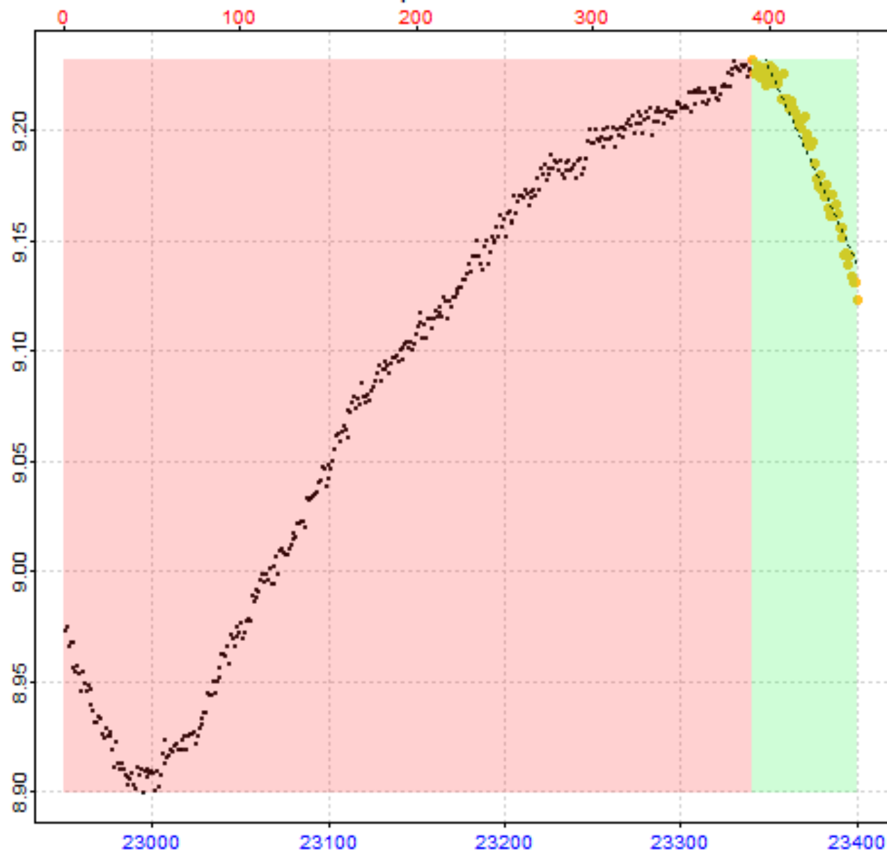
Replicate 52 of 64
