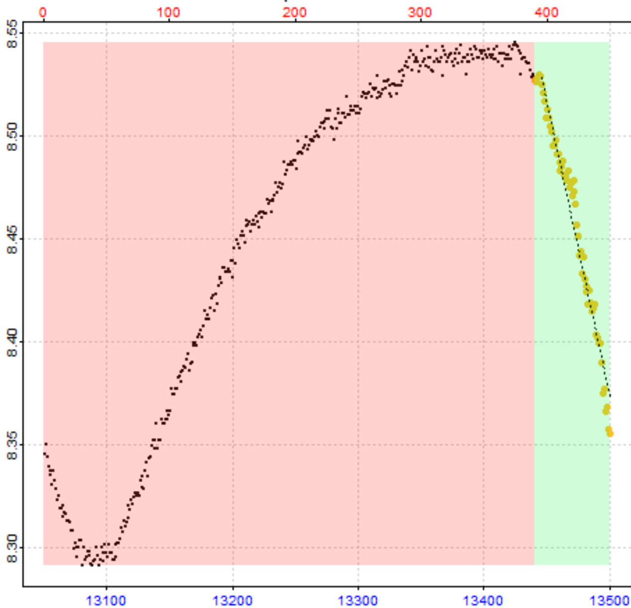
Replicate 30 of 64
