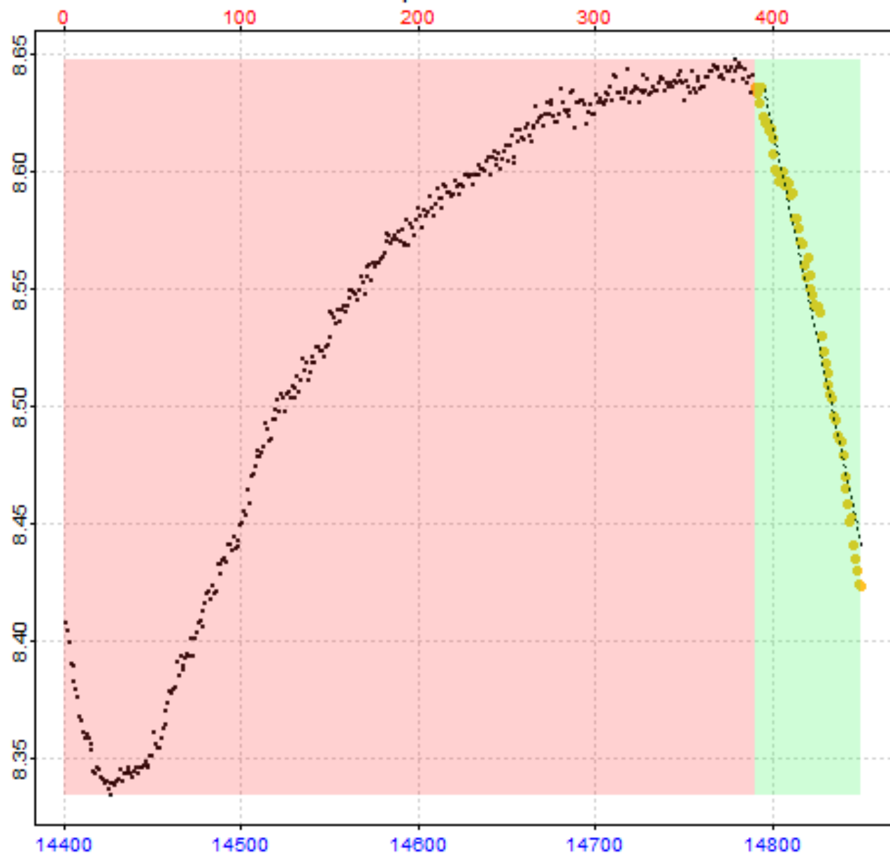
Replicate 33 of 64
