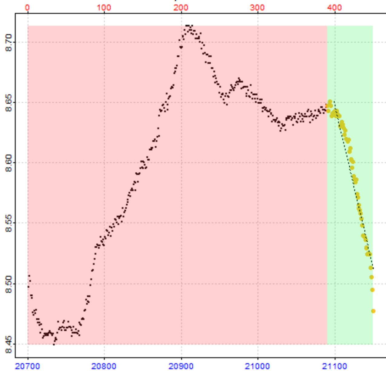
Replicate 47 of 64
