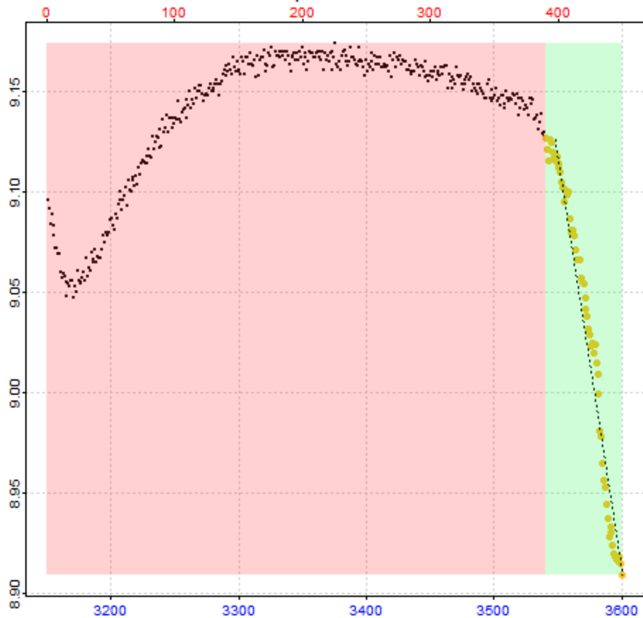
Replicate 8 of 64
