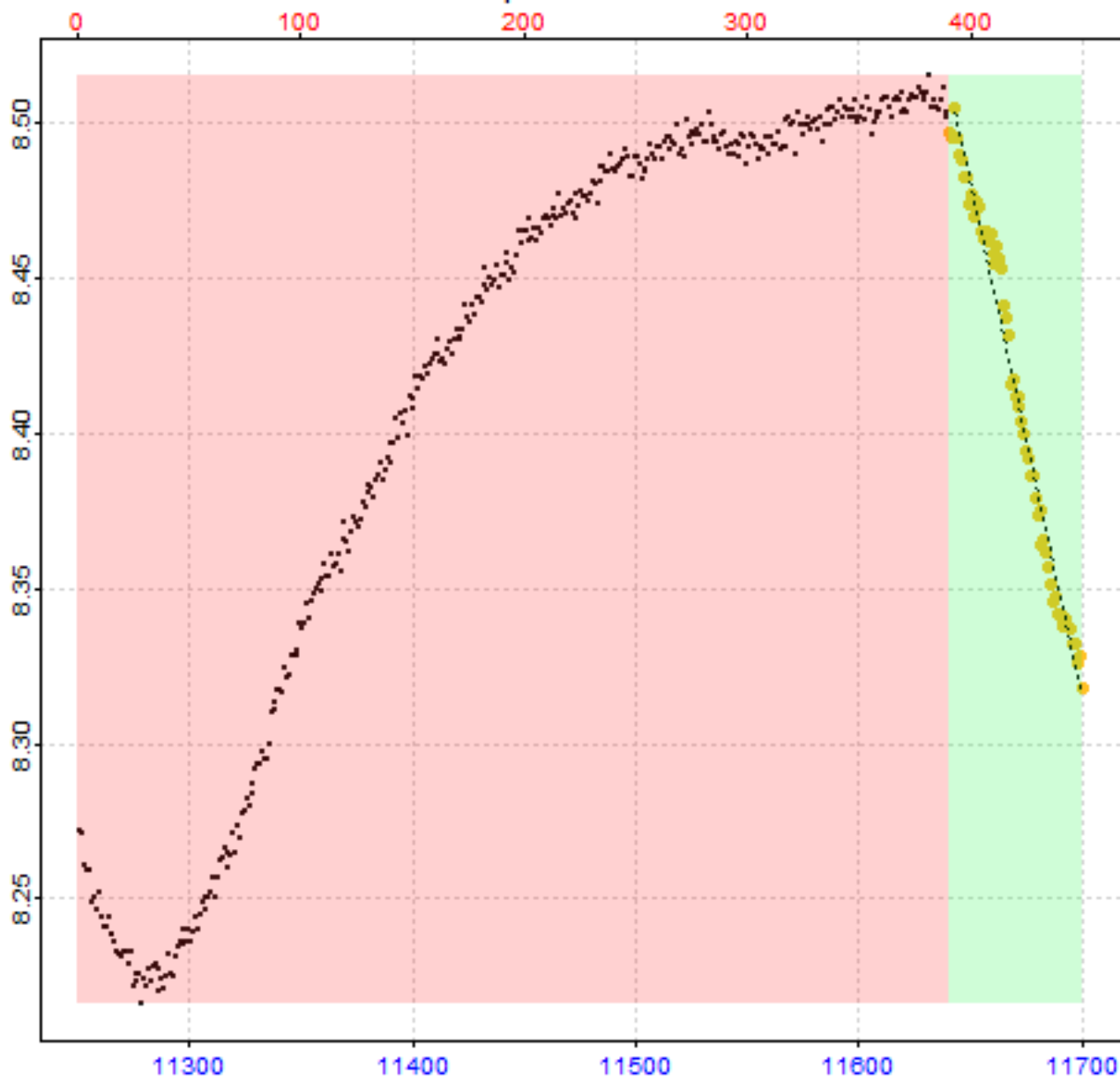
Replicate 26 of 64
