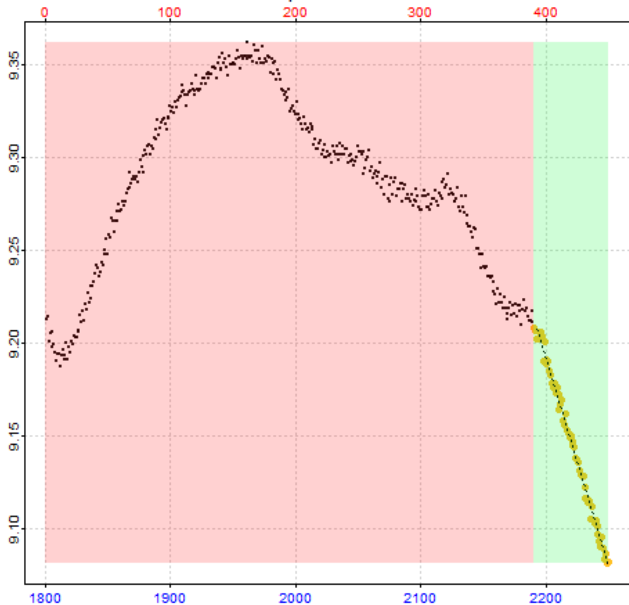
Replicate 5 of 64
