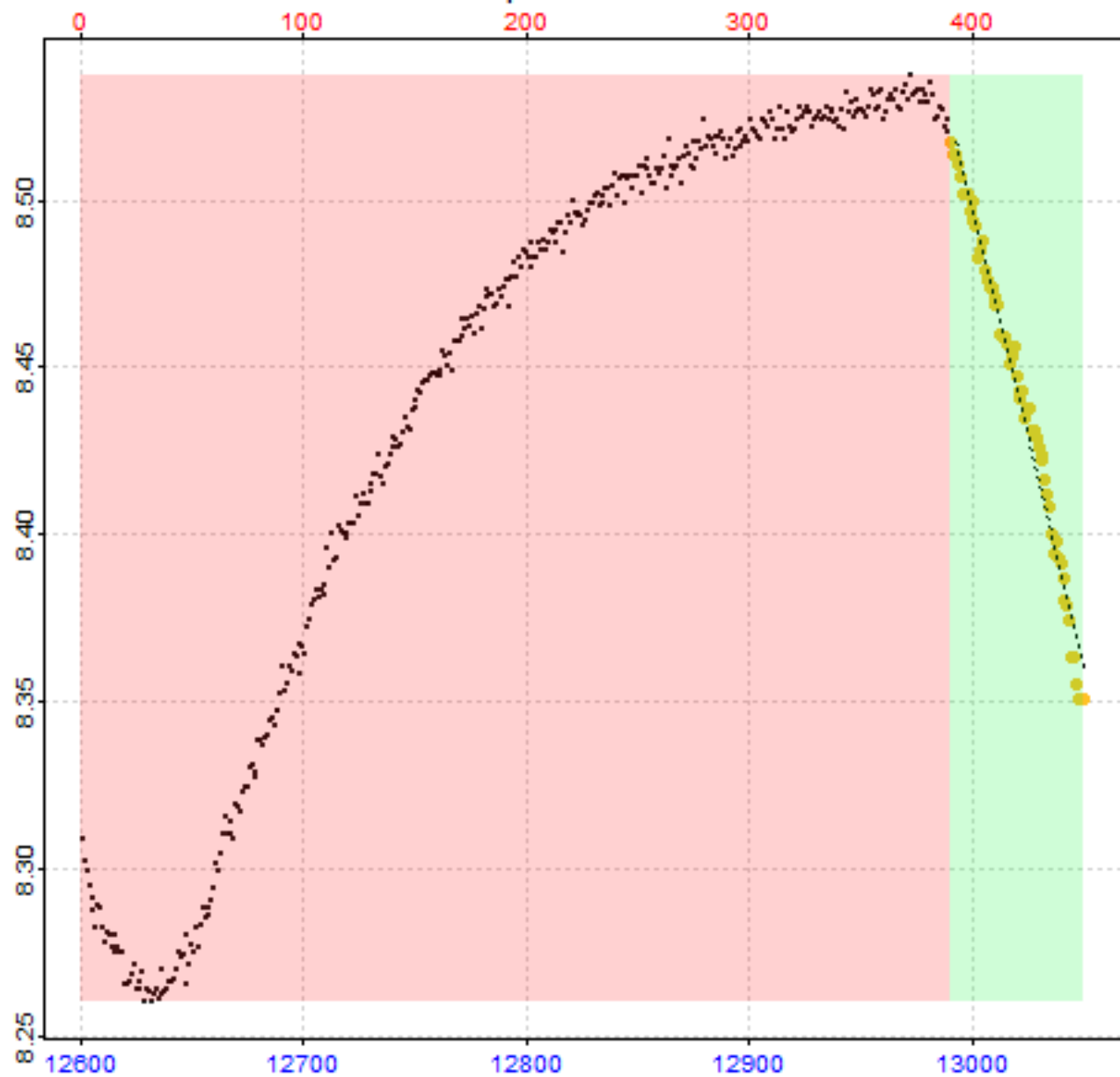
Replicate 29 of 64
