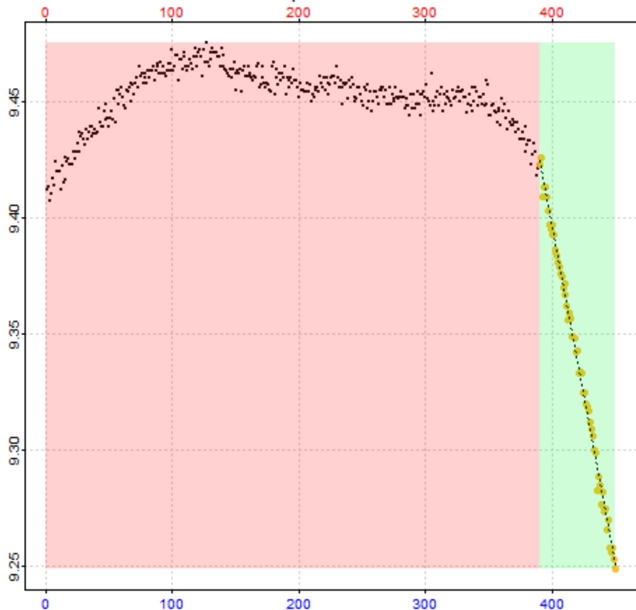
Replicate 1 of 64
