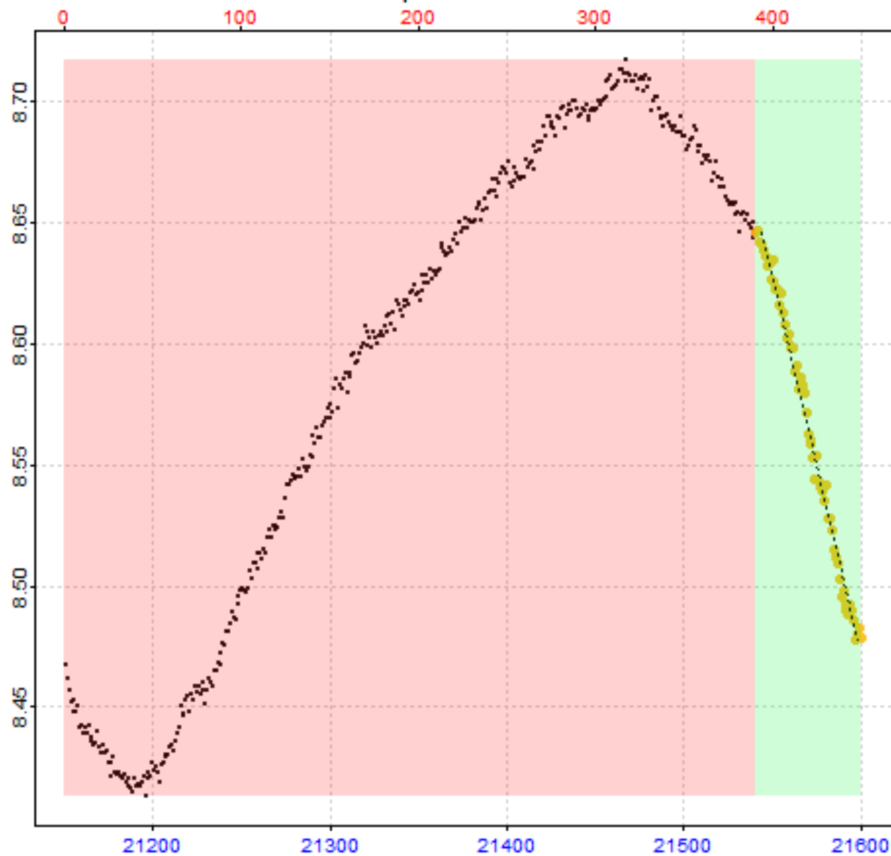
Replicate 48 of 64
