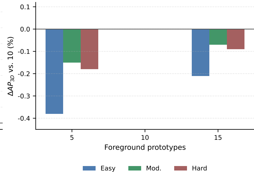
(c) Sensitivity to prototype number
