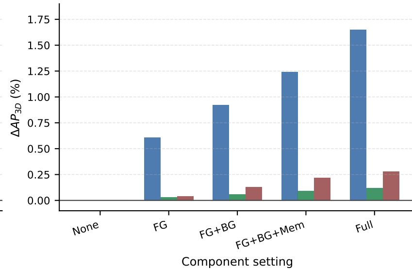
(b) Gain of prototype components
