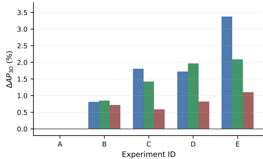
(a) Gain of main modules
