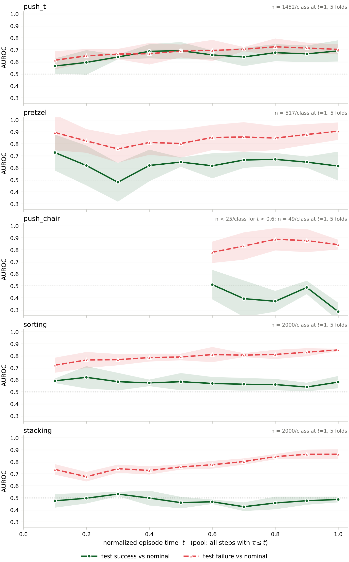
Oracle separability from nominal data: random forest on observation embeddings, grouped CV over episodes
