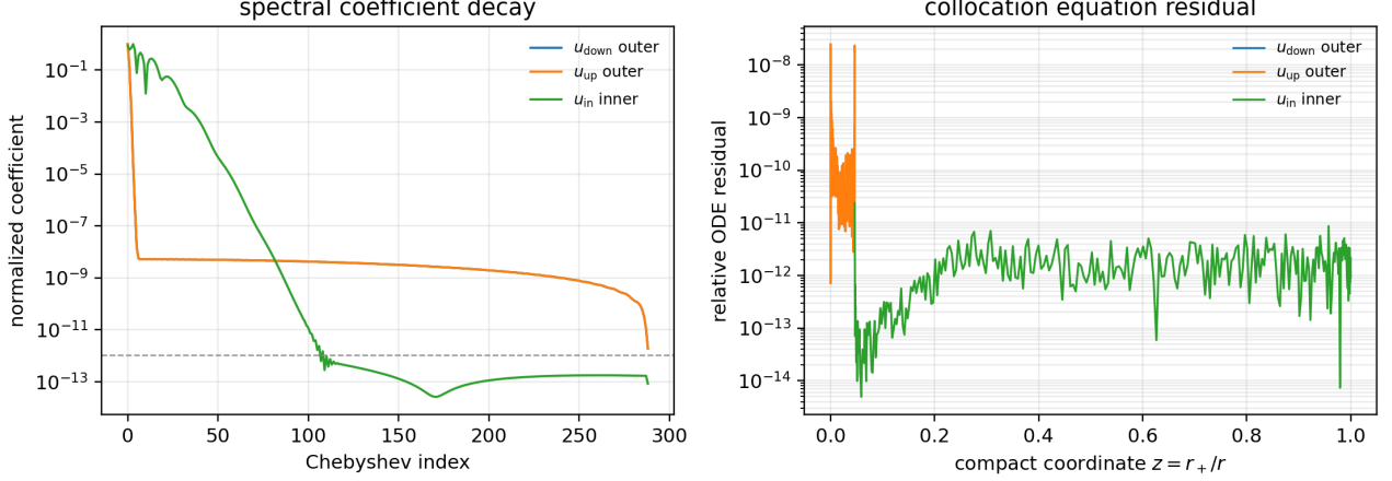
FIG. 1. Spectral quality checks for the representative Kerr mode. Left: normalized Chebyshev coefficient decay after phase peeling. Right: relative collocation-equation residuals after the computed nodal values are substituted back into the regular endpoint and interior ODE rows.
