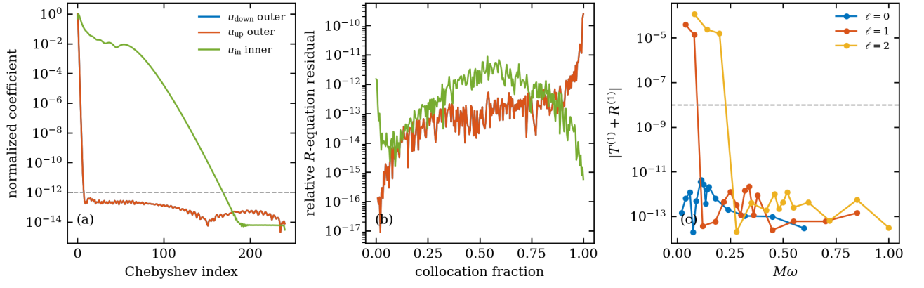
FIG. 3. Internal numerical accuracy diagnostics for the axisymmetric Kerr calculation. Panels (a) and (b) use the representative peak point a = 0.5 , m = 0 , \ell = 2 , and M\omega = 0.52 with N = 240 and quadrature order q = 192 . Panel (a) shows the normalized Chebyshev coefficients of the phase-peeled homogeneous solutions on the outer and inner subdomains. Panel (b) shows the relative residual (44) after substituting the numerical solution back into the original radial Teukolsky equation. Panel (c) shows the first-order flux-balance residual over the full axisymmetric frequency sweep. The dashed line marks the acceptance threshold 10^{-8} used in Table II.
