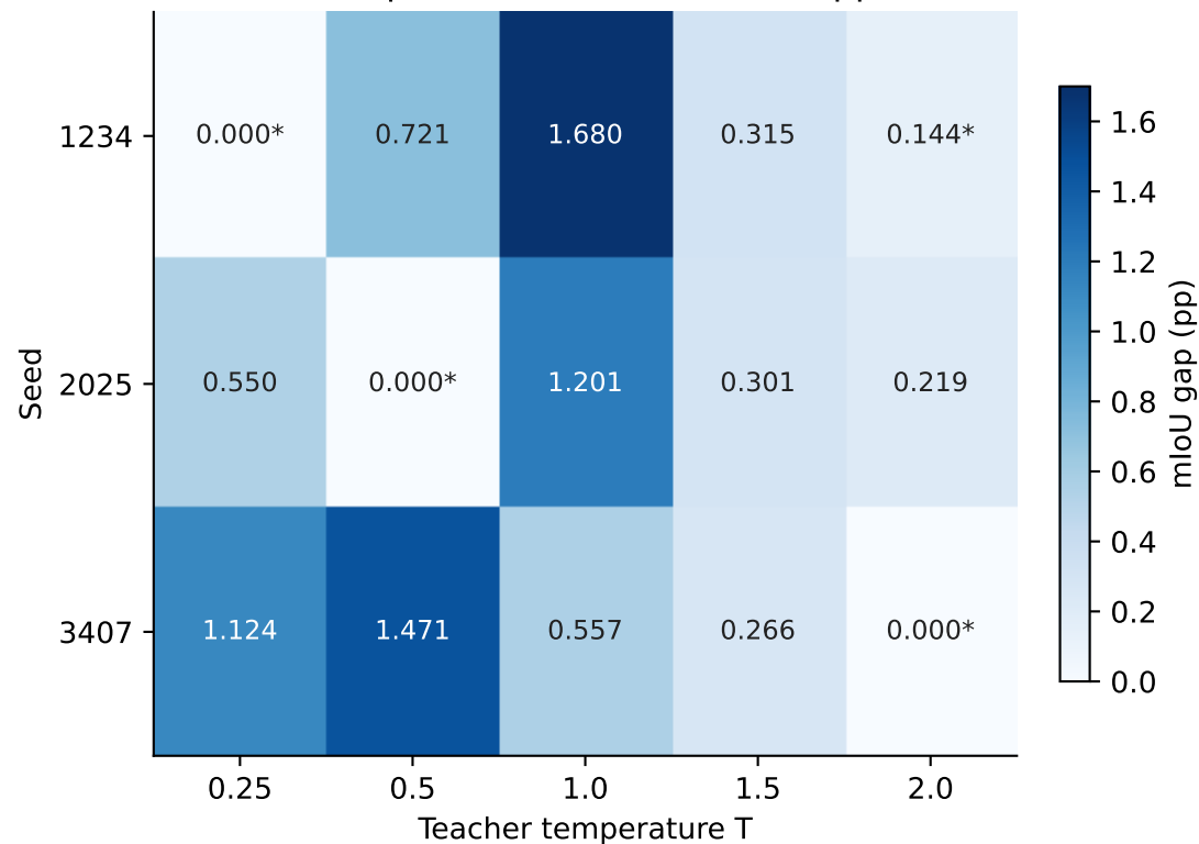
B Gap from each seed's best (pp)
