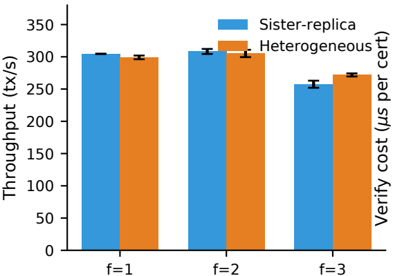
(a) Sister vs heterogeneous, NC=6
