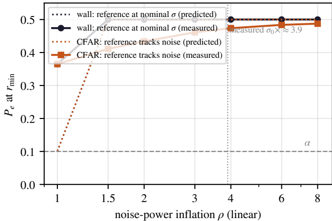
(b) \rho -scan at the frontier (BT=3840)
