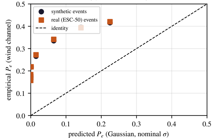
(a) real-noise mismatch
