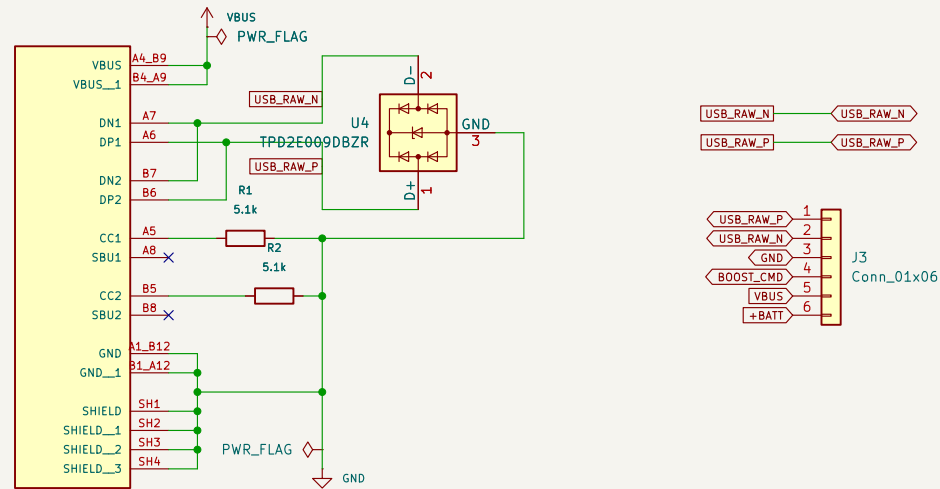
J1 USB-C (replacement daughterboard)
