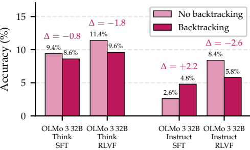
(a) Accuracy With vs. Without Backtracking
