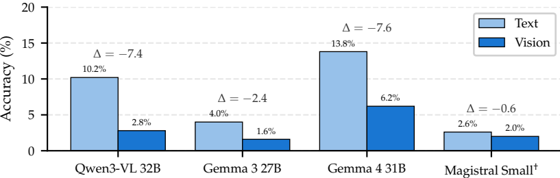
Text vs. Vision Accuracy Across Model Families
