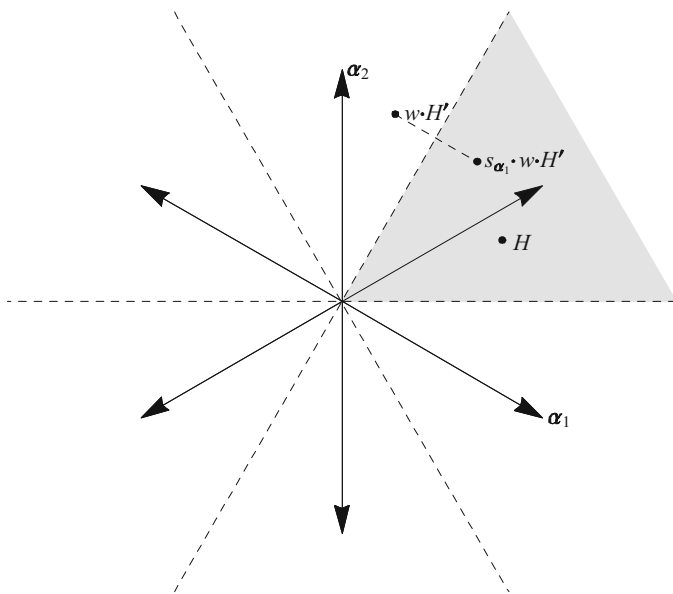
Fig. 8.9 If w \cdot H' and H are on opposite sides of the line orthogonal to \alpha_1 , then s_{\alpha_1} \cdot w \cdot H' is closer to H than w \cdot H' is
