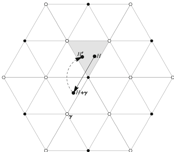
Fig. 13.6 The element \gamma is in the kernel of the exponential mapping for \text{PSU}(3) , but is not in the coroot lattice. If we apply a rotation by 2\pi/3 to H + \gamma , we obtain an element H' in the same alcove as H
