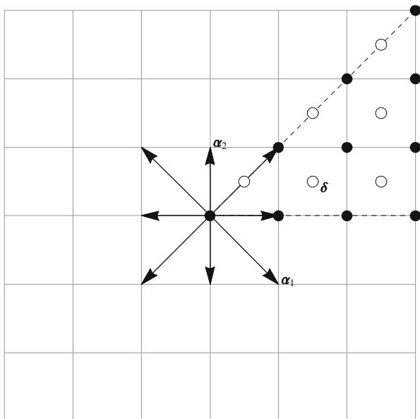
Fig. 12.3 Dominant, analytically integral elements ( black dots ) and dominant, algebraically integral elements ( black and white dots ) for \mathrm{SO}(5)
