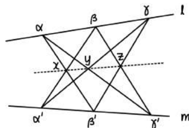
Figure 19.2 Pappus’s Theorem.
