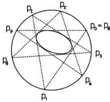
Figure 19.8 Poncelet's Porism 19.10.8.
