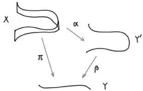
Figure 28.4 Stein factorization.
