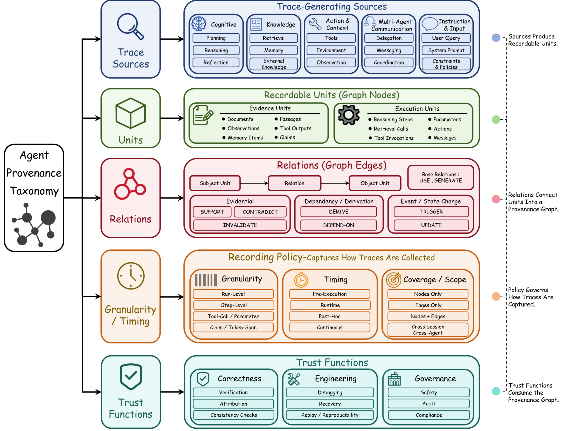
Figure 2: Taxonomy overview of agent provenance in this survey. The figure visualizes the main trace-generating components, recordable units, relations, recording policy, and trust functions; Table 1 gives the complete six-dimensional taxonomy, including representation forms.
