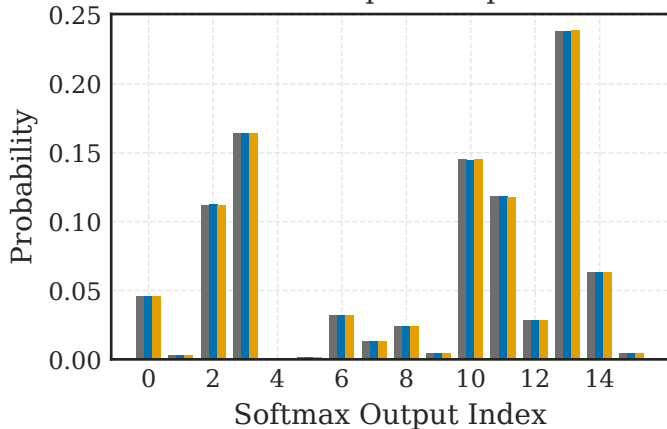
Softmax Output Comparison
