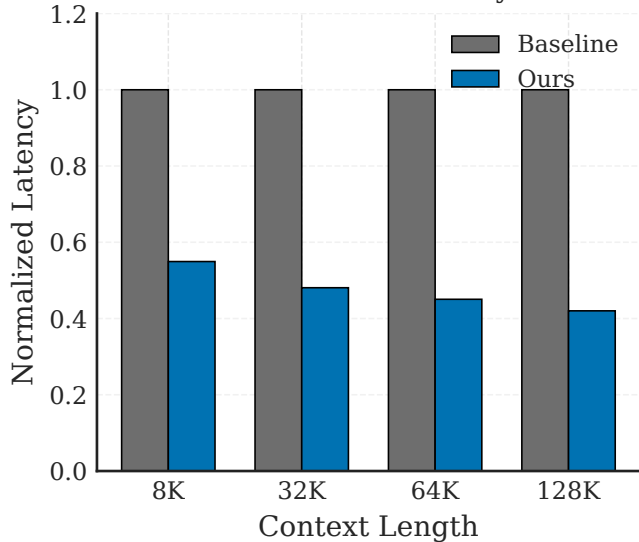
Normalized Latency
