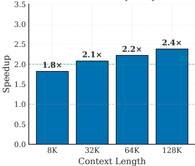
End-to-End Speedup
