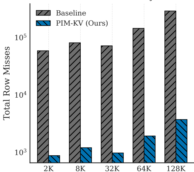
Row Buffer Locality
