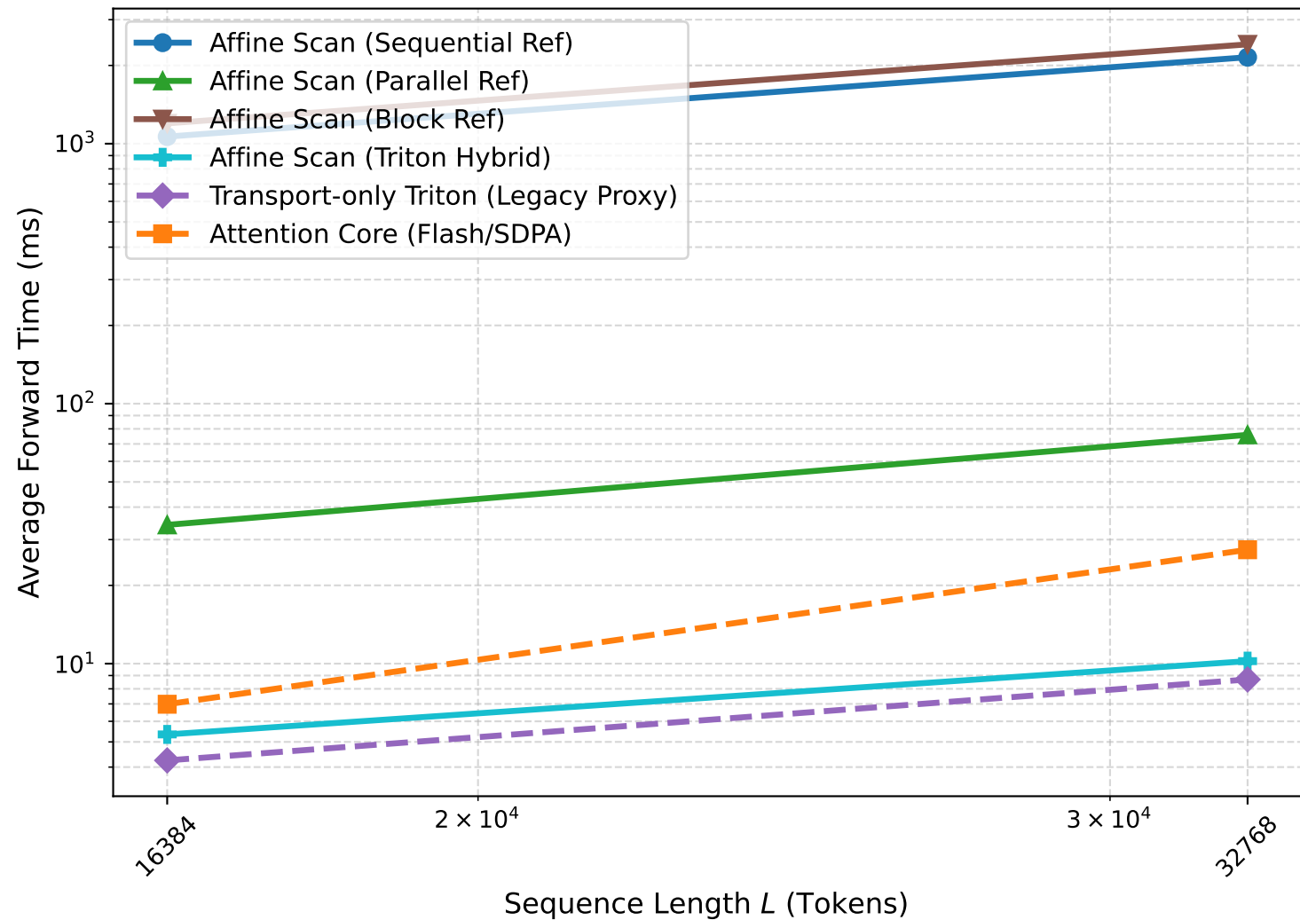
Affine Transport Core vs Attention Core (Log-Log Scale)
