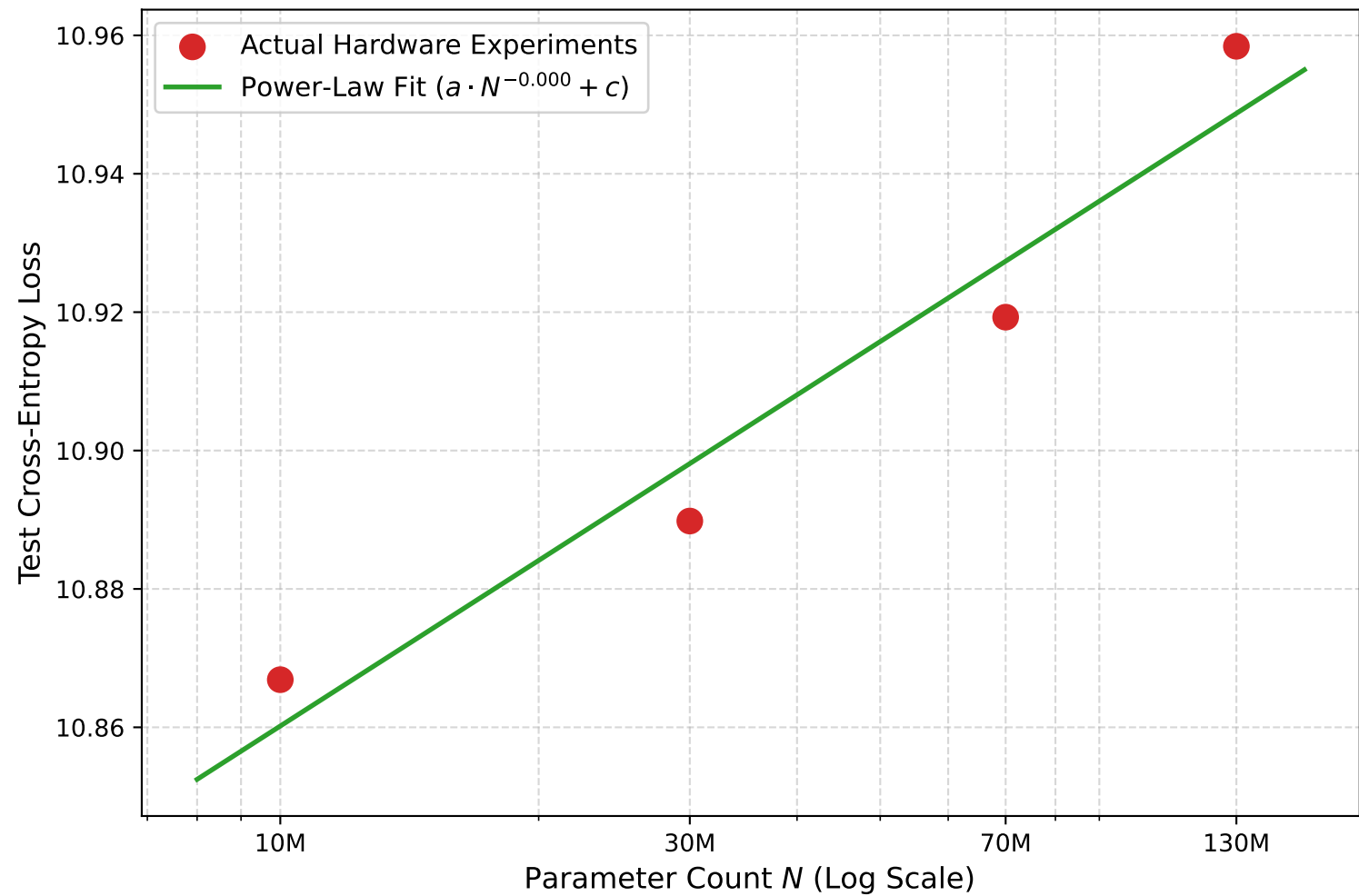
Iso-FLOP Scaling Laws of MOGT Architecture
