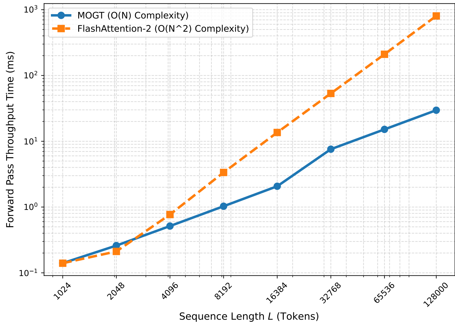
Wall-clock Time vs Sequence Length (Log-Log Scale)
