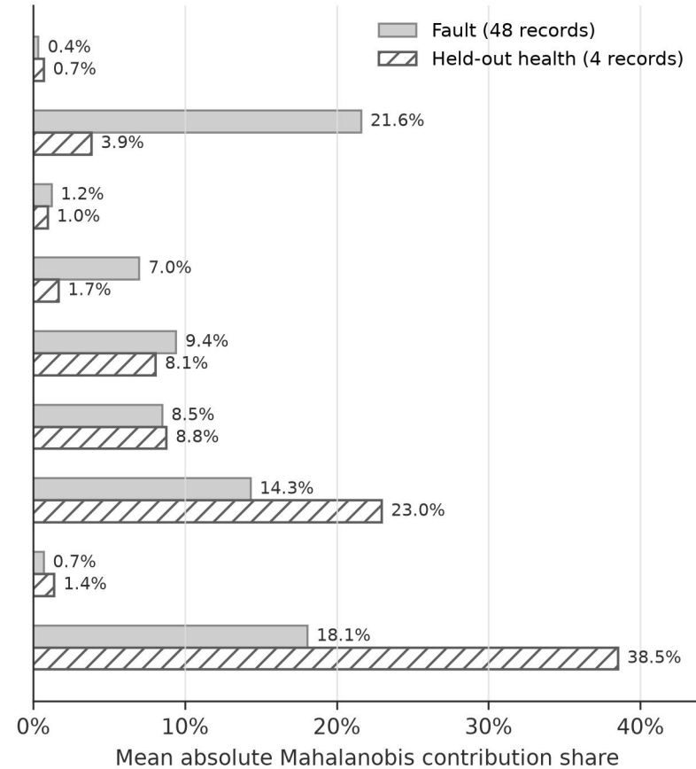
(b) Frozen-score attribution
