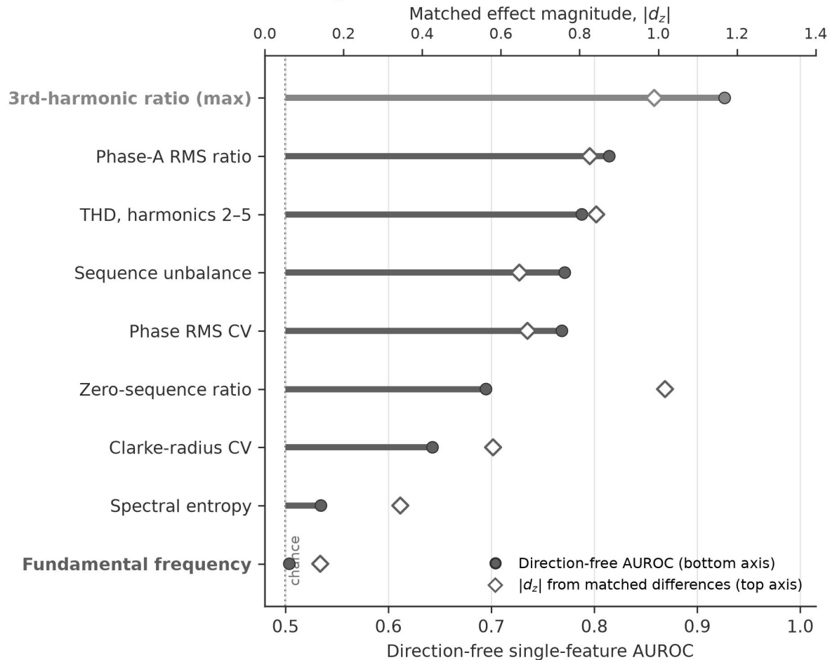
(a) Single-feature discrimination
