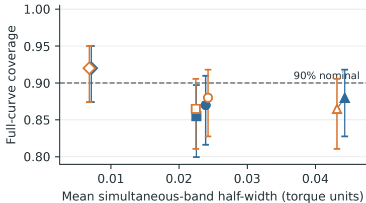
Fixed internal test (n=200)
