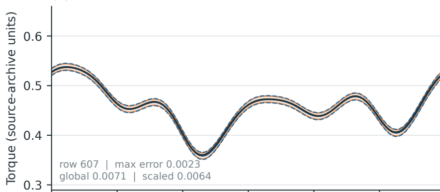
(c) Sparse uniform: both miss
