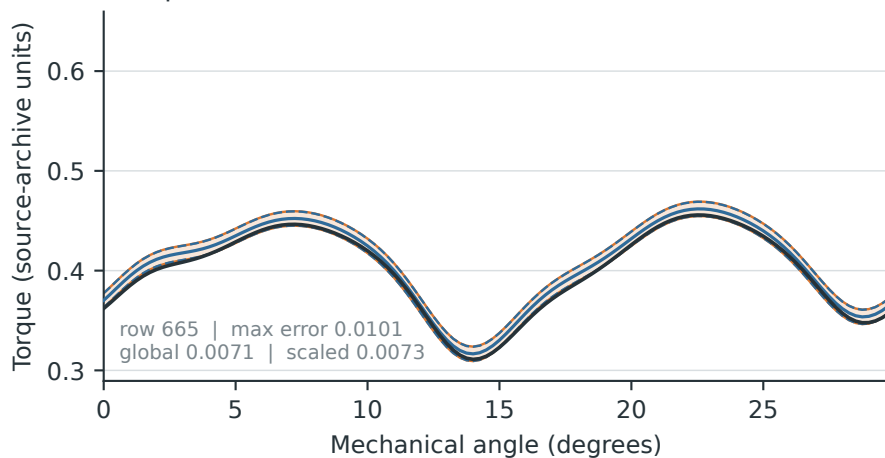
(c) Sparse uniform: both miss
