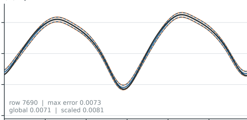
(d) Gaussian middle-density: both cover
