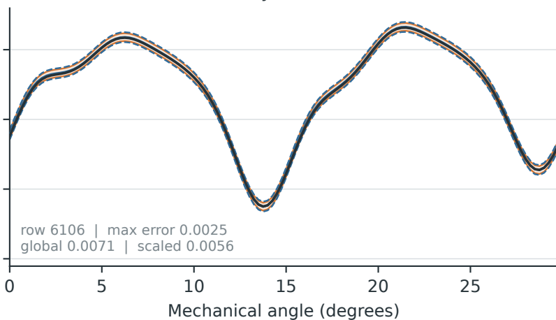
(d) Gaussian middle-density: both cover
