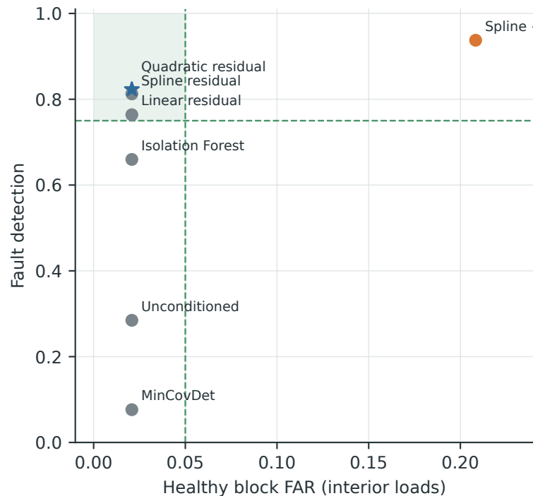
(a) Development PMSM: label-revealed selection
